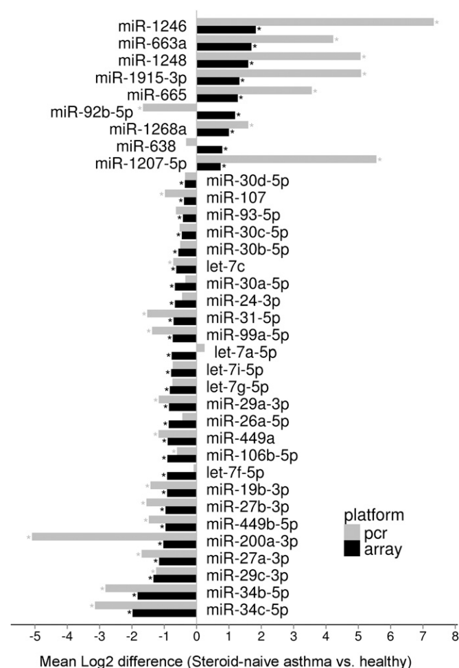
Figure 4. Polymerase chain reaction (PCR) validation of microarray findings in steroid-naive asthma. Quantitative PCR (qPCR) was used to measure 40 micro-RNA (miRNAs) selected for confirmation based on false discovery rate less than 0.01 and mean log 2 signal intensity greater than nine in microarray analyses. Five of these miRNAs did not yield detectable signal on qPCR (omitted from figure). *False discovery rate < 0.05.
