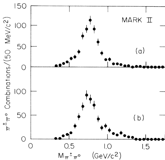
FIG. 1. The \pi^-\pi^0 invariant-mass spectrum for (a) resolved \pi^0 's and (b) unresolved \pi^0 's.
