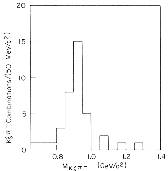
FIG. 2. The K_S^0 \pi^- invariant-mass spectrum.
