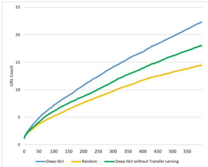
Figure 3.2: The progressive performance of Deep-GUI and random agent in web crawling. The difference between the three tools is statistically significant in all timesteps, as calculated by one tail KS-tests between all pairs (similar to the procedure described in footnote 3).
