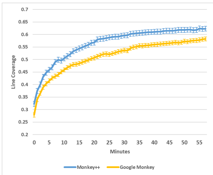
Figure 3.1: The progressive line coverage of Monkey++ and Google Monkey on the top 10 Android applications with regards to their CC
