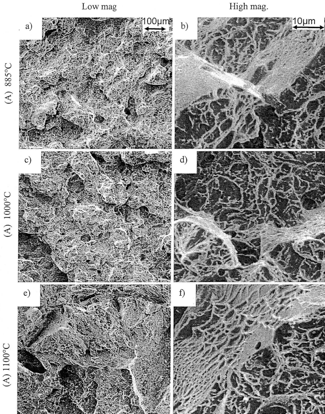
Figure 3.7 SEM fractographs of the CVN specimens of Heat #2 Test temperature: -197^{\circ}\text{C} . Cracks propagate from the bottom to the top of the images. a), b) (A) 885^{\circ}\text{C} / 26.8 \text{ J} , c), d) (A) 1000^{\circ}\text{C} / 12.9 \text{ J} , and e), f) (A) 1100^{\circ}\text{C} / 9.9 \text{ J} .
