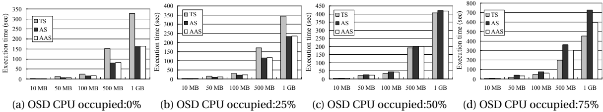
Figure 10: Execution time of processing different sizes of data when an extra process is already running in the OSD and has occupied a certain ratio of CPU (0%-75%). The application used in this experiment is Database Selection. The size of the data produced after processing is 20% of the original data. To avoid memory becomes bottleneck, we increase the physical memory of both client and OSD to 1 GB in this experiment. All the tests run with one client process and one OSD. For the Adaptive Computation Partition algorithm in AAS, the value of LOW is 0.5, and the value of HIGH is 0.7.
