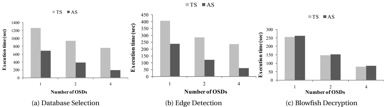
Figure 6: Execution time for different applications with different number of OSDs
