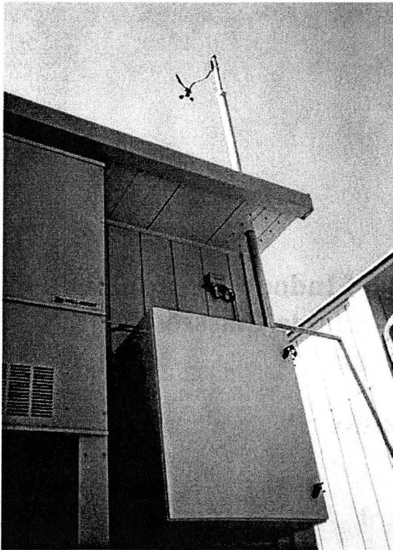
Figure 20: Photograph of the outdoor weather station to continuously measure local wind speed, wind direction, outdoor T and outdoor RH.
