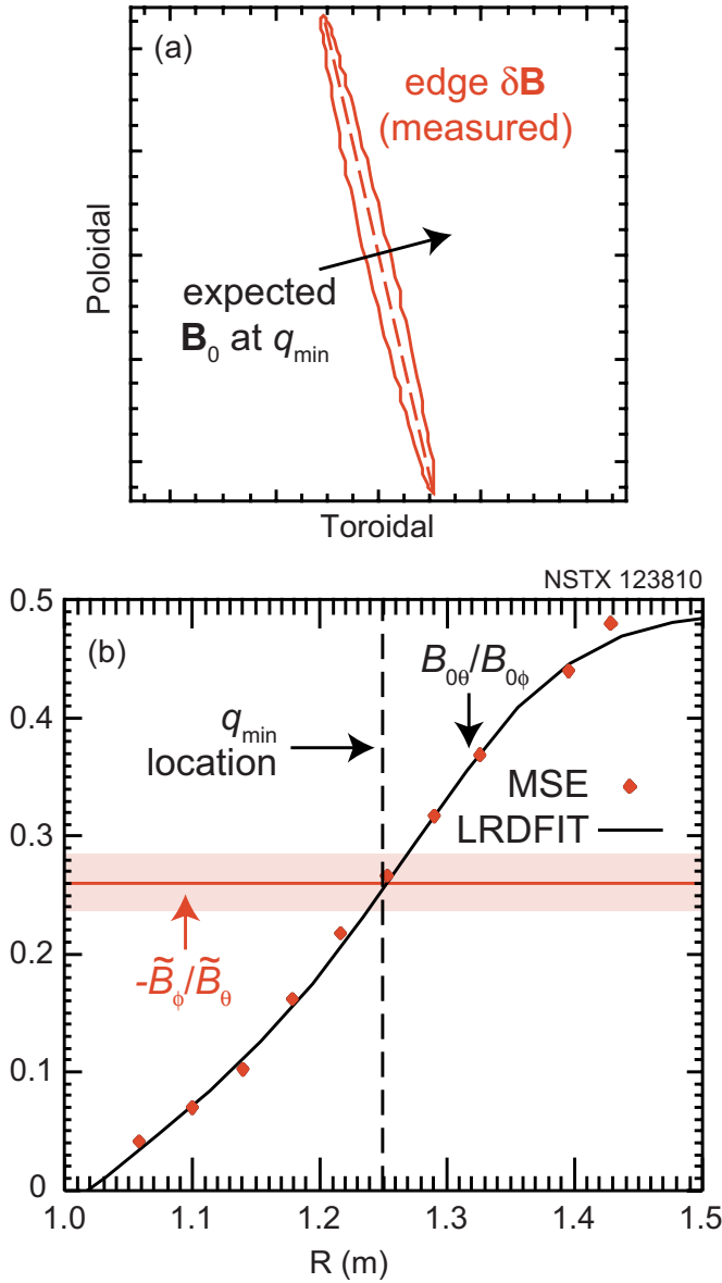
FIG. 4. (Color online) (a) \delta B_\phi vs \delta B_\theta (—) for one cycle of the n=2 AC mode (see Fig. 3), with major axis (—) and direction (→) of \mathbf{B}_0 expected at the location of minimum q ; magnitude of \delta \mathbf{B} \sim 0.6 G. (b) Comparison of equilibrium pitch B_{0\theta}/B_{0\phi} from LRDFIT (—), constrained by MSE measurements ( \blacklozenge ), with pitch required for \mathbf{B}_0 \perp \delta \mathbf{B} , which is given by -\delta B_\phi/\delta B_\theta (horizontal line). Experimental uncertainty (horizontal band) of -\delta B_\phi/\delta B_\theta and location of minimum q also shown (—).
