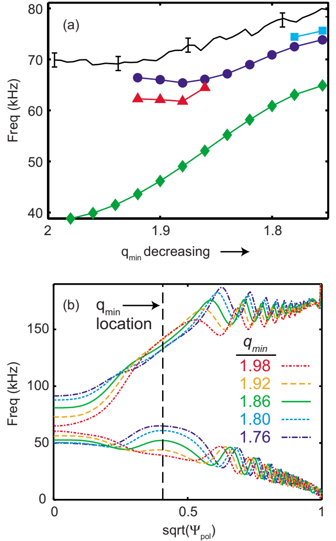
FIG. 8. (Color online) (a) Doppler corrected frequency of experimentally observed (n, m) = (2, 4) AC mode (—). Also, NOVA-K calculation of mode frequency (●), and frequency of extra modes resulting from splitting due to coupling with axis-localized AE (▲) and TAE in outboard neighboring local TAE gap (■). Frequency of continuum (◆) calculated by NOVA-K at location of minimum q . (b) Upper and lower TAE continua calculated by NOVA-K with q profile adjusted by small offsets to give different values of q_{\text{min}} . Location of minimum q is also shown (—).
