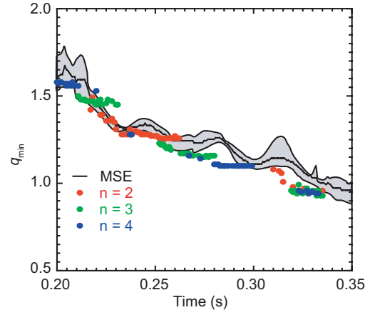
FIG. 6. (Color) q_{\text{min}} reconstructed using n=2 (red), n=3 (green), and n=4 (blue). AC modes in a low \beta plasma (shot 123099). Also shown is the average (—) and standard deviation (gray band) of q_{\text{min}} determined using MSE measurements over several very similar plasmas.
