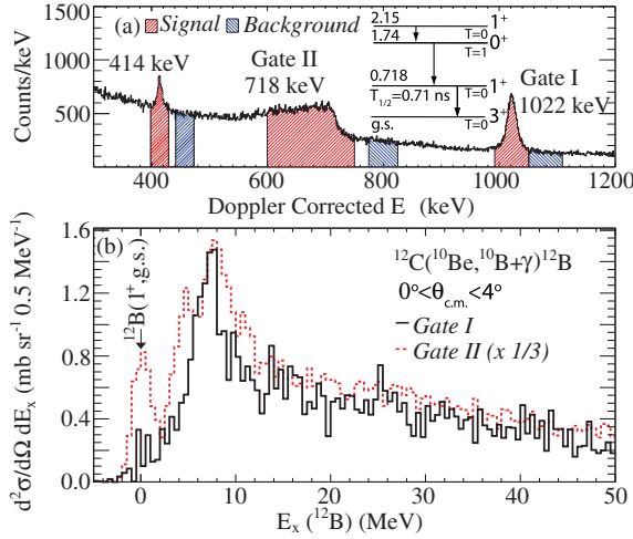
FIG. 1. (a) Doppler-reconstructed ( \beta = 0.43 ) \gamma -ray spectrum from the ^{12}\text{C}(^{10}\text{Be}, ^{10}\text{B}+\gamma) reaction. The peak at 414 keV corresponds to ^{10}\text{B}(1_2^+, 2.154 \text{ MeV}) \rightarrow ^{10}\text{B}(0_1^+, 1.740 \text{ MeV}) . The peak at 718 keV (gate II) corresponds to ^{10}\text{B}(1_1^+, 0.718 \text{ MeV}) \rightarrow ^{10}\text{B}(3_1^+, \text{g.s.}) . The peak at 1022 keV (gate I) corresponds to ^{10}\text{B}(0_1^+, 1.740 \text{ MeV}) \rightarrow ^{10}\text{B}(1_1^+, 0.718 \text{ MeV}) . (b) Sideband-subtracted double-differential cross sections gated on Gate I (solid black) and Gate II (dashed red).
