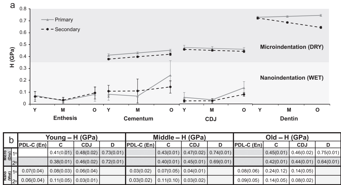
Fig. 5 – Plotted graphs (a) and table values (b, averages (standard deviations)) illustrate hardness values across the enthesis (En, PDL-cementum interface), cementum (C), cementum dentin junction (CDJ), and dentin (D). (b) An increasing trend in hardness as a function of age. Incremental changes in hardness between regions illustrate a mechanical continuum across these tissues. Notice that both cementum and dentin show similar age related trends in the apical and coronal regions while dentin exhibits an age and location interaction effect. 1° – Primary cementum and 2° – Secondary cementum.
