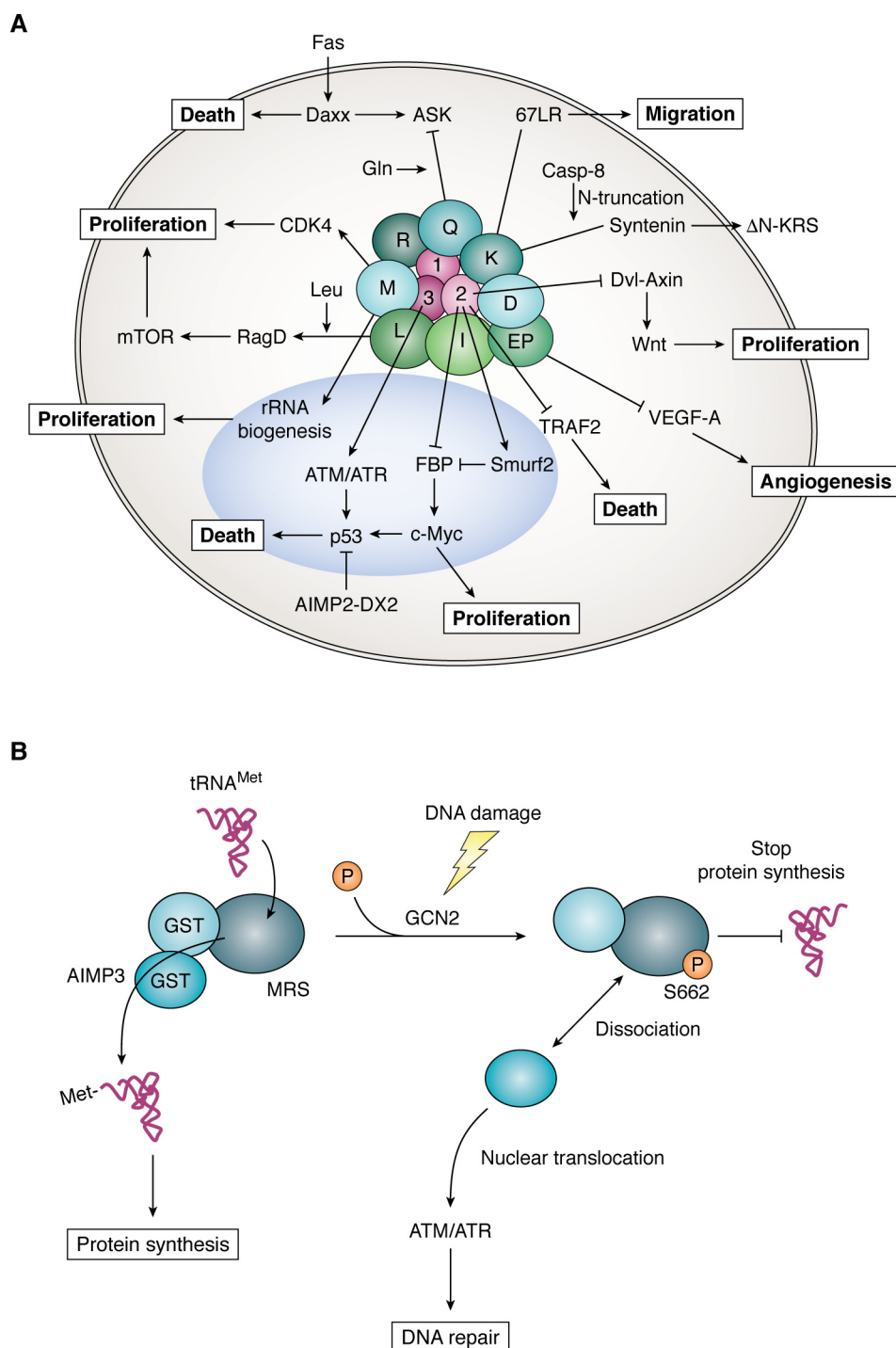
Figure 2. Signaling network of the MSC components related to protein synthesis and cancer. A, cancer-related signaling network mediated by the MSC-forming ARSs and AIMP3s. LRS functioning as a leucine sensor interacts with the RagD GTPase to stimulate the mTOR pathway (50, 51). KRS forms a metastasis-promoting interaction with the 67-kDa laminin receptor in the cell membrane (54, 55). Caspase-8 cleaves the N-terminal 12 amino acids of KRS, exposing its PDZ-binding motif at the C terminus. Syntenin binds to the exposed PDZ-binding motif of KRS and facilitates the exosome-mediated secretion of MSC-dissociated KRS (56). Induced by growth stimuli, MRS is translocated to the nucleoli to stimulate rRNA synthesis (15). MRS binds to and stabilizes CDK4 to promote the cell cycle in p16-negative cancers (57). QRS binds to apoptosis signal-regulating kinase 1 (ASK1) to regulate apoptosis in a glutamine-dependent manner (58). EPRS forms the GAIT (interferon \gamma -activated inhibitor of translation) complex with other cell factors to regulate the expression of VEGF-A mRNA (59). AIMP2 is one of three nonenzymatic factors, and it works as a potent tumor suppressor through multiple pathways, including TGF- \beta - (36), TNF \alpha - (37), Wnt- (38), and p53 (39)-mediated pathways. AIMP3 is mobilized to the nucleus by DNA damage (46, 47) or via an oncogenic stimulus (21) to activate p53 via ATM/ATR for DNA repair. B, MRS forms a complex with AIMP3 via their GST-homology domains (17). AIMP3 relays methionylated tRNA to the initiation factor to facilitate protein synthesis (11). However, upon DNA damage, MRS is phosphorylated by the activated GCN2 at the serine 662 residue that blocks tRNA Met binding, leading to the inhibition of protein synthesis (48). The dissociated AIMP3 is translocated into nucleus and activates ATM and ATR for DNA repair (21).
