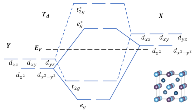
FIG. 2. Schematic of d-d orbital hybridization between the X and Y element within a half-Heusler of chemical formula XYZ . Both the X element and Y element experience tetrahedral crystal field splitting due to the C1_b crystal structure. These orbitals then hybridize according to the irreducible representations of the T_d point group. The electronegativity between the X and Y element dictates the size of the band gap.
