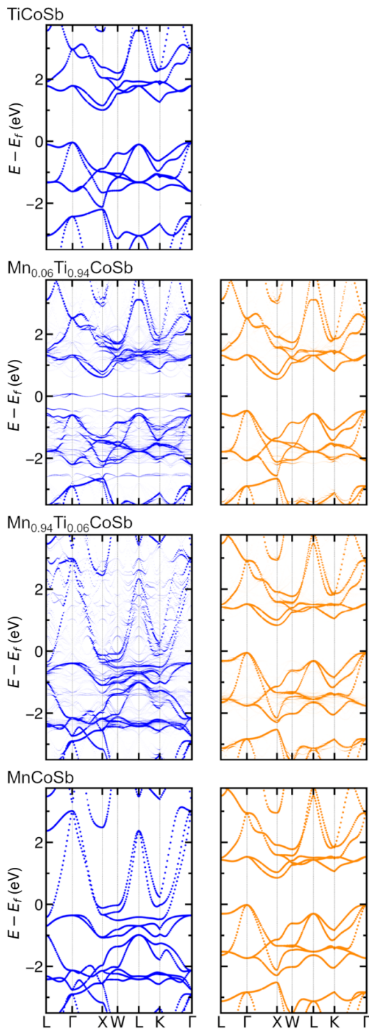
FIG. 8. Band structures of the candidate alloy system Mn_{1-x}Ti_xCoSb . The majority spin channel is shown in blue and the minority spin channel is shown in orange. The band structure of TiCoSb reflects its semiconducting nature. An indirect band gap exists between the \Gamma and X point. The introduction of a Mn solute atom within Mn_{0.06}Ti_{0.94}CoSb leads to the formation of defect electronic states that remain unhybridized with the host crystal whereas the Ti solute atom within Mn_{0.94}Ti_{0.06}CoSb only slightly disturbs the metallic majority spin channel. The band structure of MnCoSb displays half-metallic ferromagnetism.
