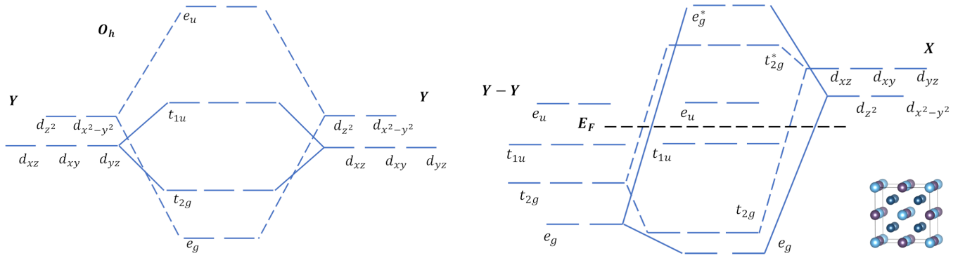
FIG. 3. Schematic of d-d orbital hybridization between both Y elements as well as X and Y elements in Heuslers with chemical formal XY_2Z . (Left) The model assumes that the d orbitals of the two distinct Y atoms, which are octahedrally coordinated by one another, hybridize first. (Right) The resulting orbitals can then hybridize with the tetrahedrally coordinated X atom of the L2_1 crystal structure. d orbital hybridization between the X atom and the Y-Y sublattice is dictated by the O_h point group which leads to a narrow band gap caused by the e_u and t_{1u} orbitals of the Y-Y sublattice that cannot further hybridize with the X atom.
