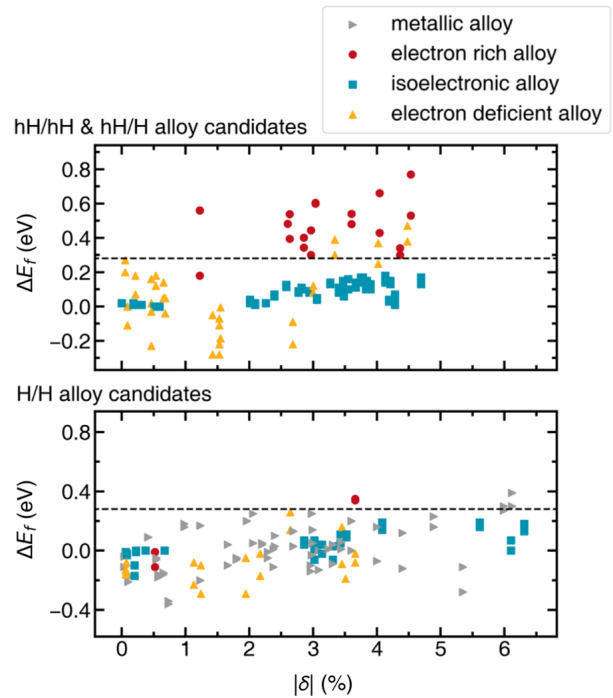
FIG. 7. (Top) The energy of formation, \Delta E_f , plotted against lattice misfit, |\delta| for all half-Heusler alloy candidates studied. The half-Heusler/Heusler alloy systems are also included here as they can be thought of as the incorporation of Y atoms of a half-Heusler with chemical formula XYZ onto the additional vacant Y sublattice. (Bottom) The energy of formation, \Delta E_f , plotted against lattice misfit, |\delta| for all Heusler alloy candidates studied. The dashed line corresponds to the qualitative upper bound for the \Delta E_f ( \Delta E_f = 0.28 eV) of an alloy in which a solid solution is expected to exist across the entire tie line
