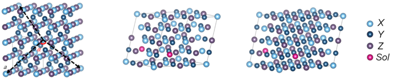
FIG. 4. (Left) The relationship between the conventional unit cell of the half-Heusler and the supercell used to calculate the energy of formations of candidate alloys. The lattice vectors of the supercell lie along the [111] directions of the conventional unit cell and are of length a and make an angle \alpha = 109.5^\circ with one another. (Center) A representative solute supercell for X -site substitution within a half-Heusler. (Right) A representative solute supercell for X -site substitution within a Heusler.
