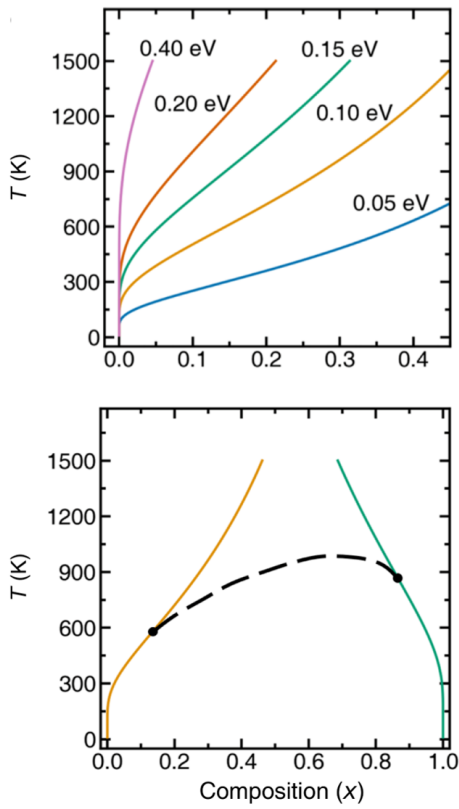
FIG. 6. (Top) The behavior of Eq. 1 for different values of \Delta E_f . For low values of \Delta E_f the solvus line dramatically breaks down at intermediate compositions. This is because Eq. 1 has an inflection point whereas real solvus lines do not. (Bottom) A model phase diagram across the tie line of two end-members. If an alloy between two half-Heuslers with chemical formula X_{1-x}A_xYZ is considered, for example, then the \Delta E_f of incorporating an A solute atom will, in general, differ from the \Delta E_f of incorporating an X solute atom. Here it is assumed that these two \Delta E_f values are 0.10 eV and 0.15 eV, respectively. The inflection points of each solvus line are marked by black circles and the dotted line connecting the two inflection points schematically depicts the anticipated behavior of the "true" solvus line at intermediate compositions.
