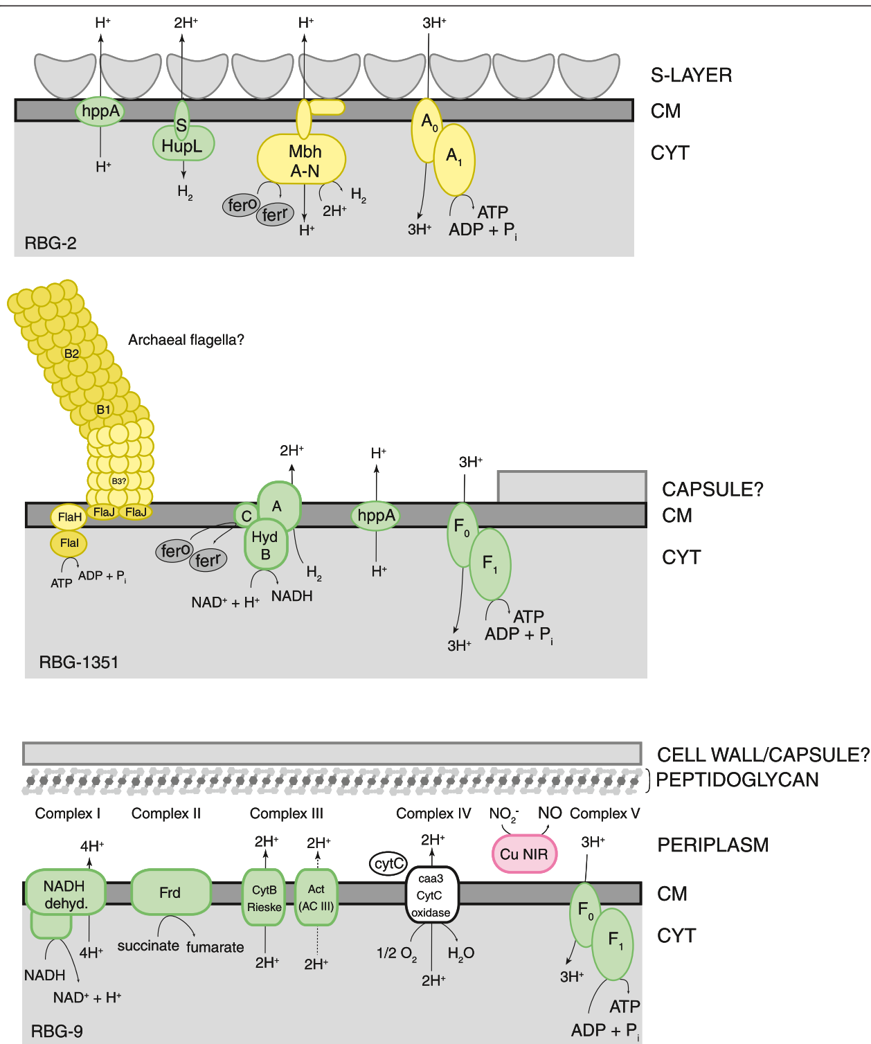
Figure 4 Predicted membrane structure and proton motive force mechanisms from the three reconstructed Chloroflexi genomes.
