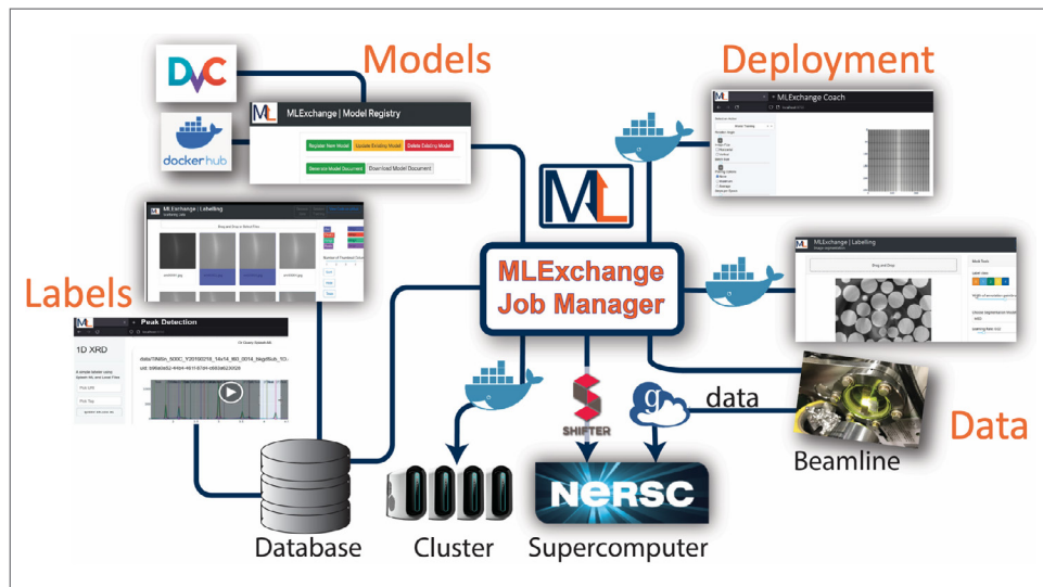
Figure 5.1.20: MLExchange project
