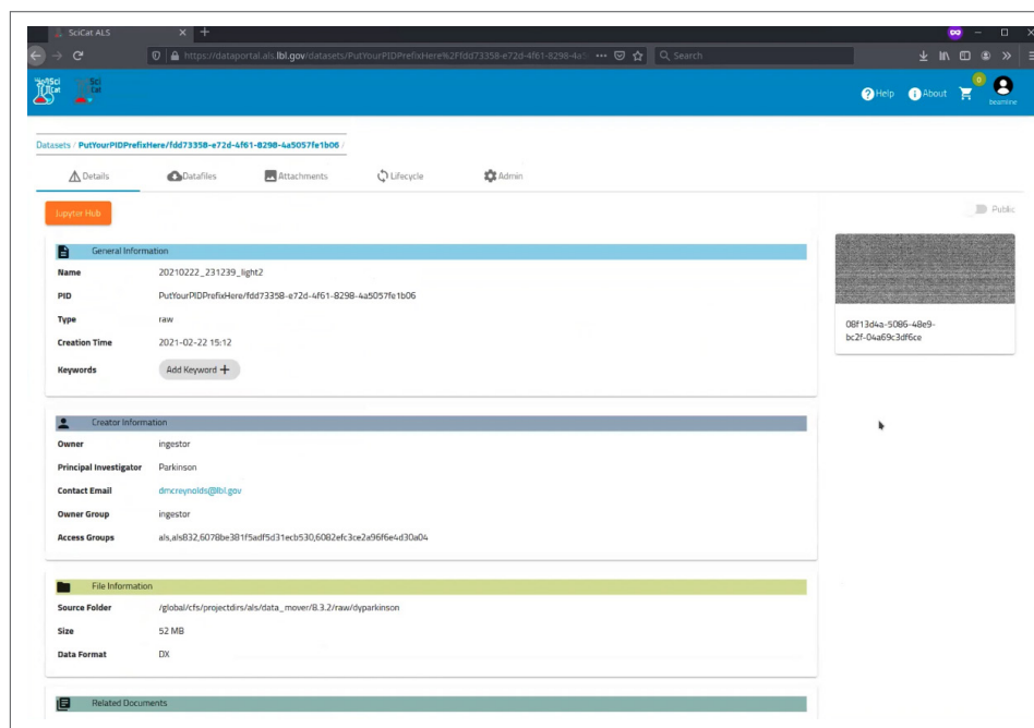
Figure 5.1.18: SciCAT
