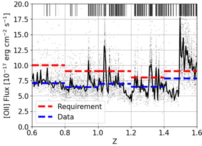
Figure 15. [O II] flux limit as a function of z_{\text{spec}} for \text{FOII\_SNR} = 7 ELG spectra. Each point marks an ELG spectrum, with the solid black line displaying the median values. The horizontal dashed blue lines are the median values for the dz = 0.2 bins, while the horizontal dashed red lines are the DESI requirements. The sky emission lines are displayed as the black rectangles at the tops of the plots, as in Figure 13. The data come from 15,400 Main ELG spectra, observed in coadded reductions with 800 \text{ s} < \text{EFFTIME\_SPEC} < 1200 \text{ s} and 6.8 < \text{FOII\_SNR} < 7.2 .
