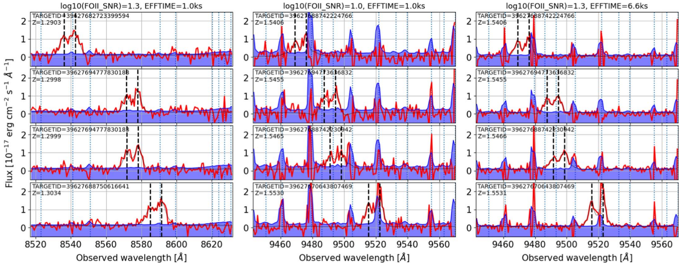
Figure 14. Illustration of the [O II] doublet in the ELG_LOP spectra. The left (middle) panel displays four spectra at z = 1.3 ( z = 1.55 ) for \text{EFFTIME\_SPEC} = 1.0 ks, with typical \text{FOII\_SNR} values for the considered redshift. The right panel displays the same four z = 1.55 targets, but as observed with \text{EFFTIME\_SPEC} = 6.6 ks. The thick red line shows the observed flux, the blue-filled region shows the flux uncertainty, and the black line is the best-fit model. The [O II] doublet wavelengths are displayed as vertical dashed black lines. The sky emission line wavelengths are indicated with the vertical blue dotted lines.
