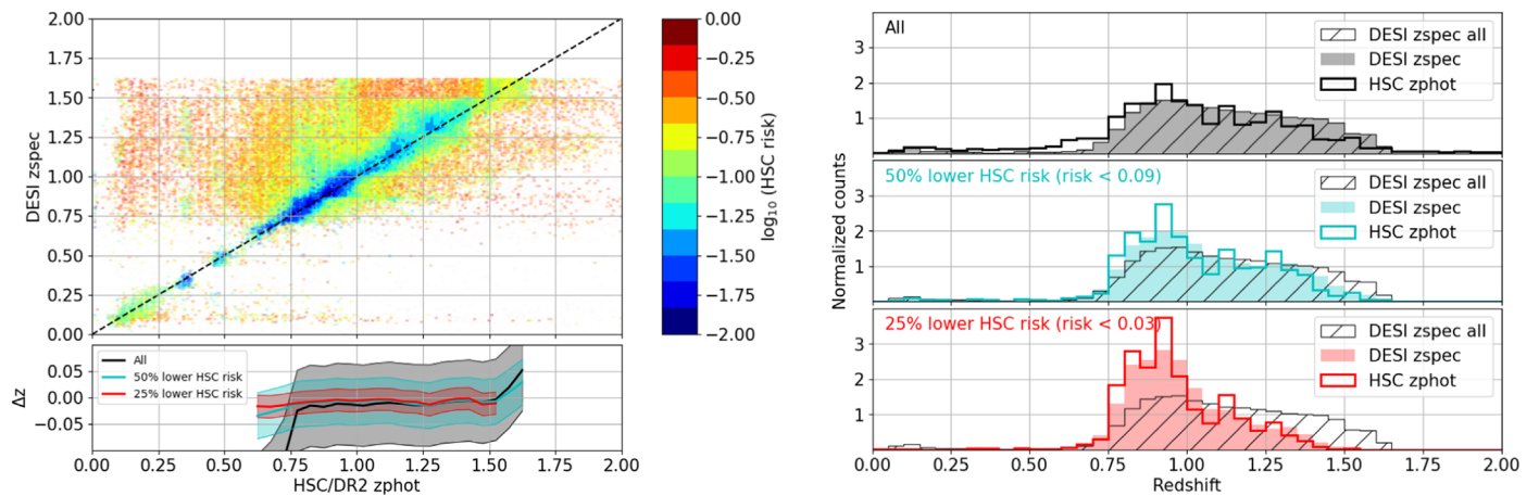
Figure B1. Comparison of the HSC/DR2 z_{\text{phot}} to the DESI Main Survey ELG z_{\text{spec}} measurements, using \sim 175,000 matched targets with a z_{\text{spec}} passing our reliability criterion of Equation (1). Left: scatter plots color-coded according to the average HSC \text{risk} parameter (see the text); the solid lines in the bottom panel are the median values of \Delta z = (z_{\text{phot}} - z_{\text{spec}})/(1 + z_{\text{spec}}) for three subsamples—all the matches (black), the 50% lower \text{risk} parameter values (cyan), and the 25% lower \text{risk} parameter values (red), with the shaded regions showing the 1.48 \times \text{MAD}(\Delta z) values. Right: redshift distributions for these three subsamples; in each panel, the filled (empty) histogram is for the DESI z_{\text{spec}} (HSC z_{\text{phot}} ). The DESI z_{\text{spec}} distribution with no cut on \text{risk} is displayed via the black hatched histogram.
