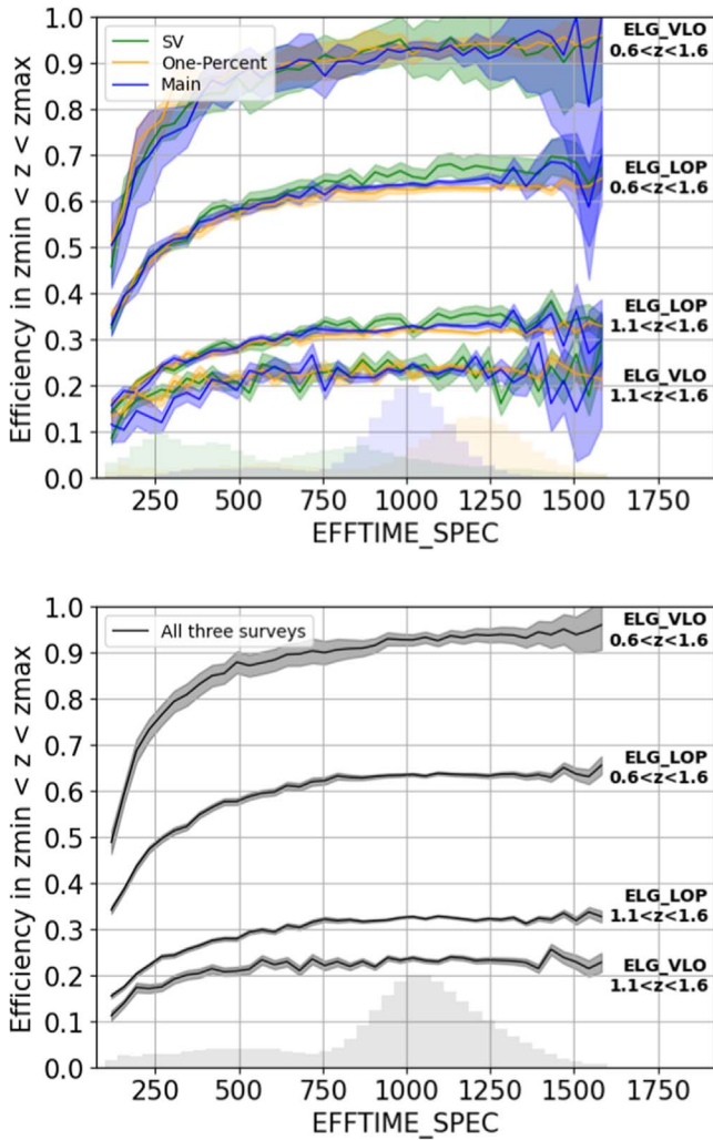
Figure 19. ELG Main selection efficiency in the 0.6 < z < 1.6 and 1.1 < z < 1.6 ranges, as a function of \text{EFFTIME\_SPEC} , for the three surveys (the SV, One-Percent, and Main Surveys). Top: split per survey. Bottom: all surveys together. The histograms show the \text{EFFTIME\_SPEC} normalized distributions.
