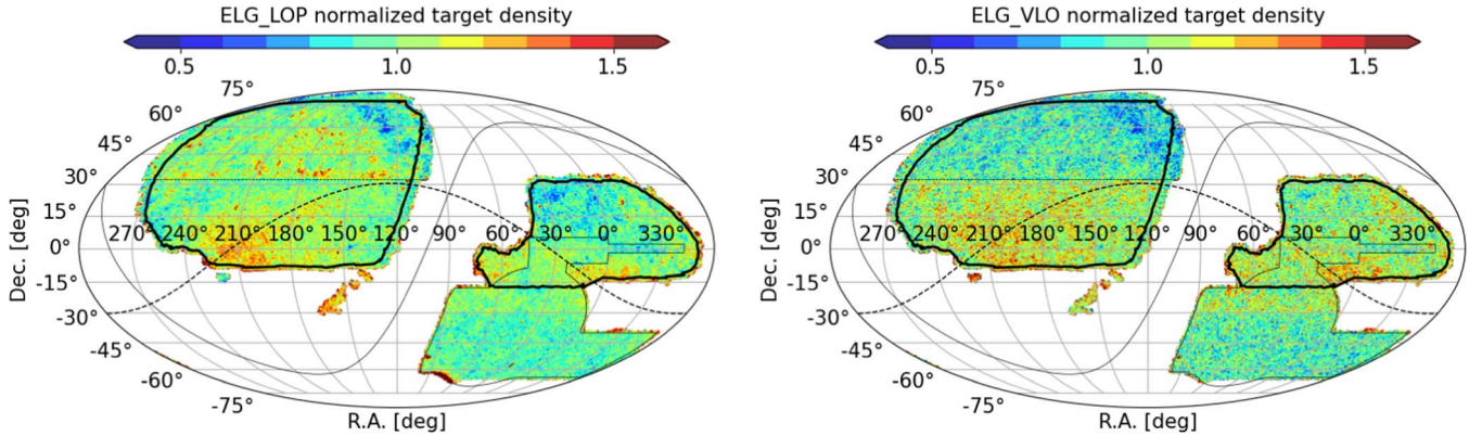
Figure 6. Main Survey ELG_LOP (left) and ELG_VLO (right) sample density sky maps. The density is divided by the overall average value ( 1940 \text{ deg}^{-2} for the ELG_LOP sample and 460 \text{ deg}^{-2} for the ELG_VLO sample), to display the fractional difference to the average. The thick black line represents the 14,000 \text{ deg}^2 footprint covered by DESI. The Galactic plane is displayed as a solid line, while the Sagittarius plane is displayed as a dashed line.
