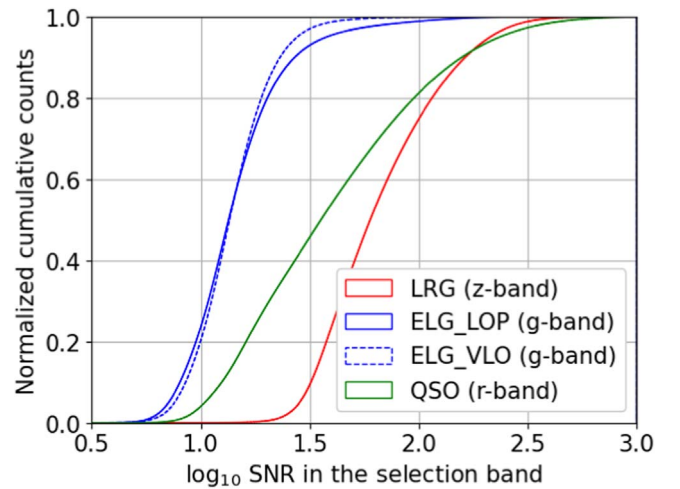
Figure 2. Cumulative distribution of the logarithm of the photometric S/N (see the text) in the selection band for the DESI Main Survey dark tracers over the nominal DESI footprints. For the ELG targets, the two Main Survey selections are shown.
