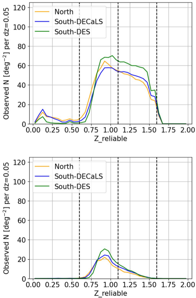
Figure 21. Redshift distributions for the Main ELG_LOP (top) and ELG_VLO (bottom) samples, split by footprint. The reported densities are the expected densities of the observed ELG targets providing a reliable z_{\text{spec}} (see the text for more details). The vertical dashed lines emphasize the relevant redshift ranges for the ELGs: z = 0.6 , z = 1.1 , and z = 1.6 .
