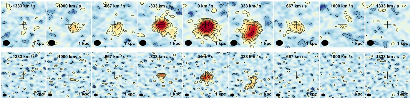
Figure 3. CO J(2 \rightarrow 1) maps of SDSS J1341–0321 averaged over 333 \text{ km s}^{-1} channels spanning \Delta V = \pm 1500 \text{ km s}^{-1} (labels give channel centers) relative to the systemic redshift. The top row shows the naturally weighted images, and the bottom row shows the Briggs ( R = 0 ) weighted images. Contours start at 2\sigma and are logarithmically spaced at 0.2 dex multiples of \sigma . Dashed contours are negative equivalents. The crosshair indicates the peak of the stellar emission in the HST /F814W imaging (Figure 1). Black ellipses show the FWHM of the synthesized beam.
