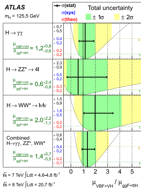
Fig. 8. Measurements of the \mu_{VBF+VH}/\mu_{ggF+ttH} ratios for the individual diboson final states and their combination, for a Higgs boson mass m_H = 125.5 \text{ GeV} . The best-fit values are represented by the solid vertical lines, with the total \pm 1\sigma and \pm 2\sigma uncertainties indicated by the dark- and light-shaded band, respectively, and the statistical uncertainties by the superimposed horizontal error bars. The numbers in the second column specify the contributions of the statistical uncertainty (top), the total (experimental and theoretical) systematic uncertainty (middle), and the theoretical uncertainty (bottom) on the signal cross section (from QCD scale, PDF, and branching ratios) alone. For a more complete illustration, the distributions of the likelihood ratios from which the total uncertainties are extracted are overlaid.
