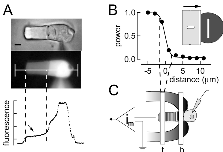
Figure 1. Experimental patch dialysis design and characterization of slit width. (A) Bright field and fluorescence images of a salamander rod dialyzed for 2 min with Lucifer yellow by patch pipette. The line drawn down the central axis of the rod indicates the regions from which pixels were selected, and fluorescence was plotted as a function of distance. The region designated between the dashed lines is the outer segment. After 2 min of dialysis, this region's fluorescence indicates relatively even loading. Bar, \sim 5 \mu\text{m} . (B) Measurement of light slit. The power of light that passed through the slit gradually declined as a function of the distance from its edge; this was measured by passing a razor blade from left to right immediately under it and between it and a photo detector. The smooth black curve is a sigmoid curve fitted to the data points. Dashed lines are drawn indicating the drop in power from 90 to 10%, providing an estimate of the fall of light intensity beyond the nominal edge of the slit of \sim 3.5 \mu\text{m} . Inset depicts the slit measurement arrangement as seen from above.
