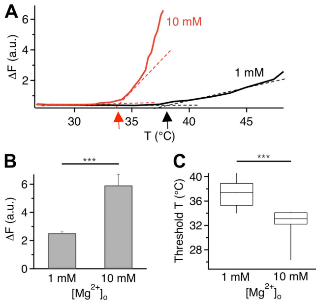
Figure 8. Shift in TRPV1 heat activation measured by fluorescence imaging. (A) Change in fluorescence intensity as a function of temperature in the presence of 1 mM (black) or 10 mM (red) \text{Mg}^{2+} . Arrows indicate the activation threshold temperature. (B) Comparison of heat-induced fluorescence increases at two \text{Mg}^{2+} concentrations. Error bars indicate \pm SEM. (C) \text{Mg}^{2+} significantly lowers the activation threshold temperature. ***, P < 0.001 ; n = 58 (for 1 mM \text{Mg}^{2+} ) and 28 (for 10 mM \text{Mg}^{2+} ).
