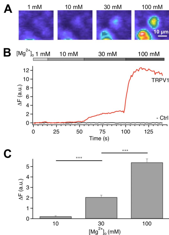
Figure 2. Mg^{2+} induces Ca^{2+} influx in TRPV1-expressing cells. (A) Live-cell fluorescence imaging of changes in intracellular Ca^{2+} concentration. (B) Representative time courses of the fluorescence signal in a channel-expressing cell and an untransfected cell. Changes in fluorescence intensity are shown in arbitrary units after subtracting the basal level intensity. (C) Change in fluorescence intensity increases with Mg^{2+} concentration. ***, P < 0.001 ; n = 70 –113. Error bars indicate \pm SEM.
