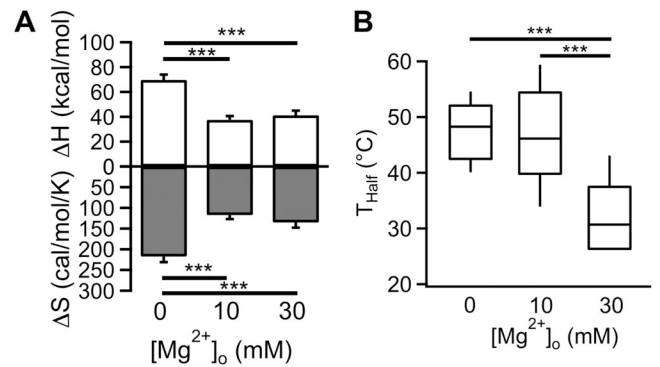
Figure 9. Thermodynamic analysis of \text{Mg}^{2+} effects on heat activation. (A) Measured \Delta H values (open bars) and \Delta S values (shaded bars) from heat-induced currents. Error bars indicate \pm SEM. (B) Box-and-whisker plot of the half-activation temperature T_{\text{half}} at the corresponding \text{Mg}^{2+} concentration. ***, P < 0.001 ; n = 5-6 .
