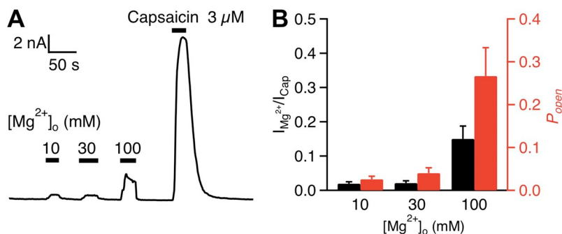
Figure 3. \text{Mg}^{2+} activates TRPV1 current in a dose-dependent manner. (A) Representative whole-cell currents at +80 mV evoked by \text{Mg}^{2+} and capsaicin. (B) Mean currents (black bars) evoked by \text{Mg}^{2+} normalized to the response evoked by 3 \mu\text{M} capsaicin (left axis). The red bars represent the same data after correction for \text{Mg}^{2+} inhibition of the single-channel conductance (see Fig. 4), so that the height of the bars directly reflects relative open probability (right axis). n = 5 each. Error bars indicate \pm\text{SEM} .
