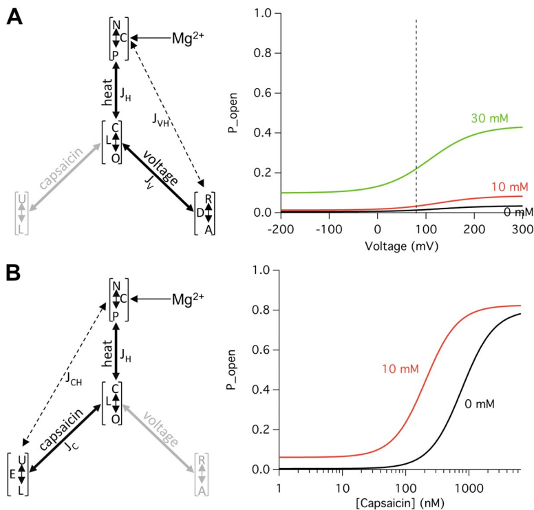
Figure 11. \text{Mg}^{2+} potentiation of heat activation can substantially affect voltage- and capsaicin-dependent activation. All simulations were generated using values derived from experimental data presented in Figs. 3, 5, 6, and 9, and the following parameters: L = 0.005 , J_H = 300 , J_V = 7 , J_C = 800 , J_{VH} = 1 , and J_{CH} = 1 . (A) \text{Mg}^{2+} effects on voltage-dependent activation. (left) The dual-allosteric model containing the heat and voltage branches, with \text{Mg}^{2+} affecting the equilibrium constant C. (right) Predicted voltage-dependent activation using Eq. 5. The broken line indicates the position of +80 mV. (B) \text{Mg}^{2+} effects on capsaicin-dependent activation. (left) The dual-allosteric model containing the heat and capsaicin branches, with \text{Mg}^{2+} affecting the equilibrium constant C. (right) Predicted capsaicin dose-response curves using Eq. 6.
