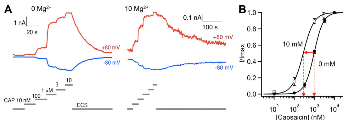
Figure 6. Effects of \text{Mg}^{2+} on the capsaicin-dependent activation of TRPV1. (A) Representative whole-cell current traces in response to varying capsaicin concentration in the absence (left) or presence (right) of 10 mM \text{Mg}^{2+} . (B) Dose-dependent activation of TRPV1 by capsaicin in the absence (closed circles) or presence (open circles) of 10 mM \text{Mg}^{2+} . Curves represent fits of a Hill equation. The EC_{50} and slope factor values are: 977 \pm 15 nM and 1.88 \pm 0.05 ( n = 3 ) for 0 mM \text{Mg}^{2+} , and 282 \pm 20 nM and 1.61 \pm 0.10 ( n = 4 ) for 10 mM \text{Mg}^{2+} . Error bars indicate \pm SEM.
