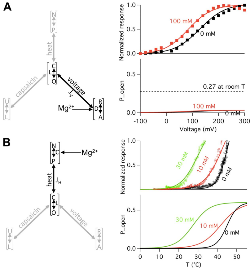
Figure 10. Identification of the \text{Mg}^{2+} target in the multi-allosteric TRPV1 gating model. All simulations were generated using values derived from experimental data presented in Figs. 3, 5, 6, and 9, and the following parameters: L = 0.005 , J_H = 300 , and J_V = 7 . (A) Effects of \text{Mg}^{2+} on channel open probability through the voltage-dependent branch. (left) The voltage-dependent branch of the gating pyramid, with \text{Mg}^{2+} affecting the equilibrium constant D . (right, top) Normalized P - V curves in the absence (black curve) or presence (red curve) of 100 mM \text{Mg}^{2+} . Superimposed are experimentally determined G - V relationships (closed squares). (right, bottom) Predicted channel open probabilities using Eq. 3. The maximal open probability level in the presence of 100 mM \text{Mg}^{2+} is significantly lower than the experimental observation (indicated by the broken line), which is \sim 27\% at +80 mV and room temperature (see Fig. 3 B). (B) Effects of \text{Mg}^{2+} on channel open probability through the heat-dependent branch. (right, top) Predicted heat dependence in the absence (black curve) or presence of 10 mM (red curve) or 30 mM (green curve) \text{Mg}^{2+} . Superimposed are experimentally determined I - T relationships (circles). (right, bottom) Predicted channel open probabilities using Eq. 4.
