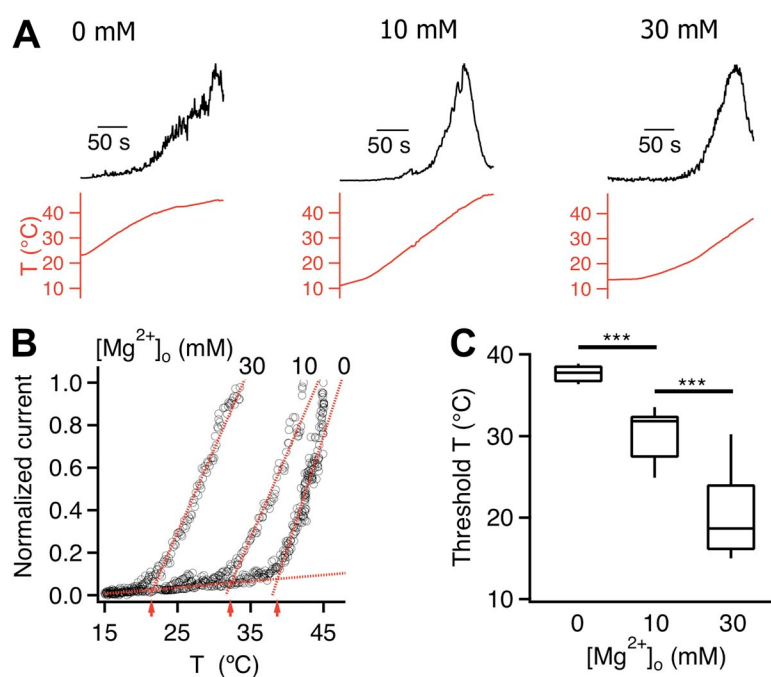
Figure 7. \text{Mg}^{2+} strongly potentiates the temperature response of TRPV1. (A) Normalized current (top) induced by a temperature ramp (bottom) recorded from inside-out patches at +80 mV with 0 mM, 10 mM, and 30 mM \text{Mg}^{2+} in the pipette solution. Recordings are from three separate patches. (B) The current raising phase is shown as a function of temperature. The activation threshold temperatures, at the intersection of a pair of dotted lines (representing the leak current and the heat-activated TRPV1 current), are indicated by red arrows. (C) \text{Mg}^{2+} dose-dependently lowered the activation temperature. ***, P < 0.001 ; n = 8-9 .
