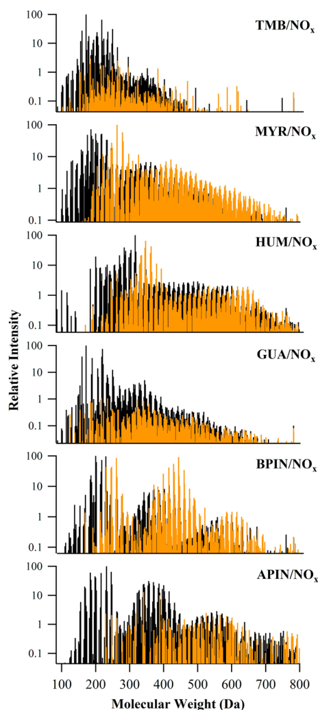
Figure 3. Reconstructed mass spectra for all VOC/NO x SOA samples (before photolysis) recorded in this work. The x -axis corresponds to the molecular weight of the neutral SOA compounds. The y -axis is on a log scale to make the weaker peaks of oligomeric compounds easier to see. Peaks in orange denote nitrogen-containing compounds.
