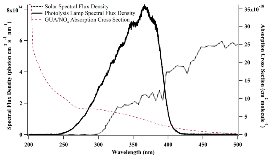
Figure 1. Spectral flux density in the photolysis cuvette compared to the solar spectral flux density at SZA = 0. The right axis shows the effective absorption cross-sections of GUA/NO x calculated from eq 1.
