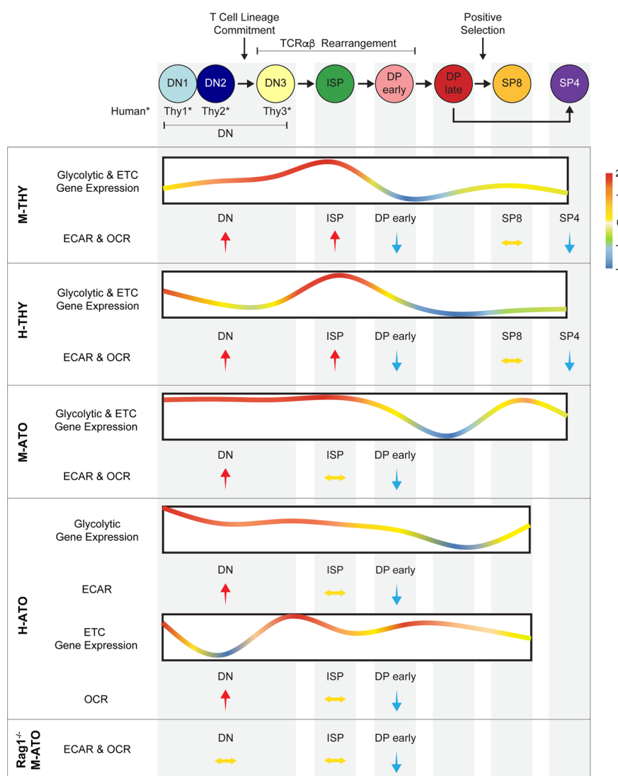
FIGURE 8 | Schematic summarizing metabolism dynamics throughout thymocyte development in M-THY, H-THY, M-ATO, H-THY, H-ATO, and RAG1 -/- M-ATO. Glycolytic and ETC gene expression patterns are represented with line plots. Color scale indicates relative fold change. Relative changes in extracellular flux between thymocyte populations are represented with arrows. H-ATO glycolytic and ETC results are shown separately. (*DN populations are named DN1-3 in mouse, and Thy1-3 in human.)
