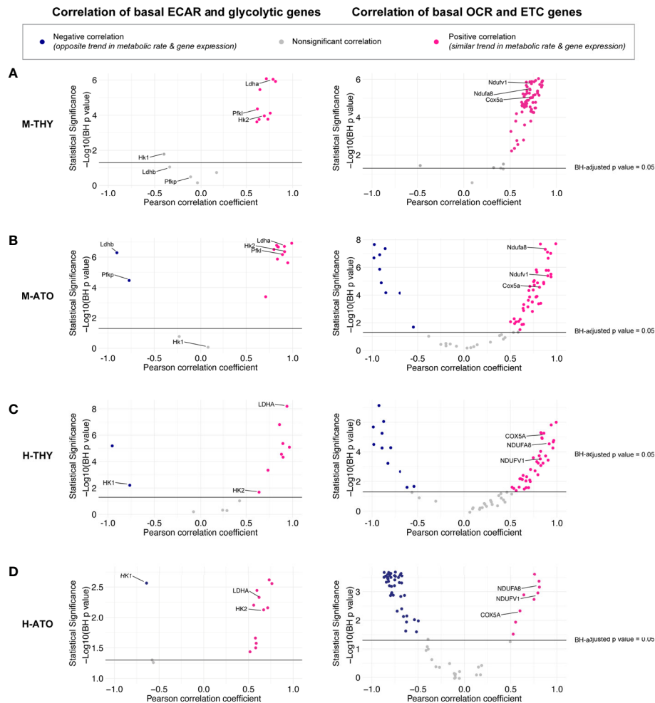
FIGURE 5 | (A–D) Scatter plots show correlation between (left) glycolytic enzyme gene expression and basal glycolysis (ECAR), or (right) correlation between electron transport chain gene expression and basal respiration (OCR) in (A) M-THY, (B) M-ATO, and (C) H-THY, and (D) H-ATO. The x axis represents the Pearson correlation coefficient R values calculated for individual genes within the specified metabolic pathway for all cell populations for which respective extracellular flux data was collected. The y axis represents the statistical significance of each R value using -\log_{10} of Benjamini-Hochberg adjusted p-values. Solid black line indicates an adjusted p-value of 0.05; all R values above the line are statistically significant. Genes with R values >0.5 (pink) are positively correlated with metabolic flux data, while genes with R values <-0.5 (blue) are negatively correlated with metabolic flux data. Nonsignificant or weak correlation R values >-0.05 or <0.5 are indicated in grey. Certain genes of interest are indicated. (M-THY: n=6 flux analysis values for 5 populations, n=2 RNA-seq replicates; H-THY: n=3 flux analysis values for 5 populations, n=3 RNA-seq replicates; M-ATO: n=6 flux analysis values for 3 populations, n=2 RNA-seq replicates; H-ATO: n=6 flux analysis values for 3 populations, n=2 RNA-seq replicates).
