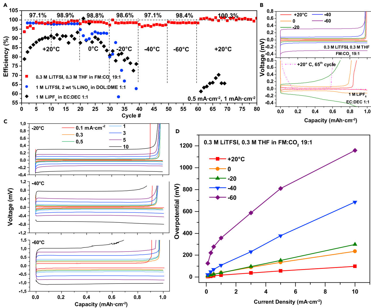
Figure 3. Li-Metal Low-Temperature Electrochemical Performance in Liquefied Gas Electrolyte (original)
