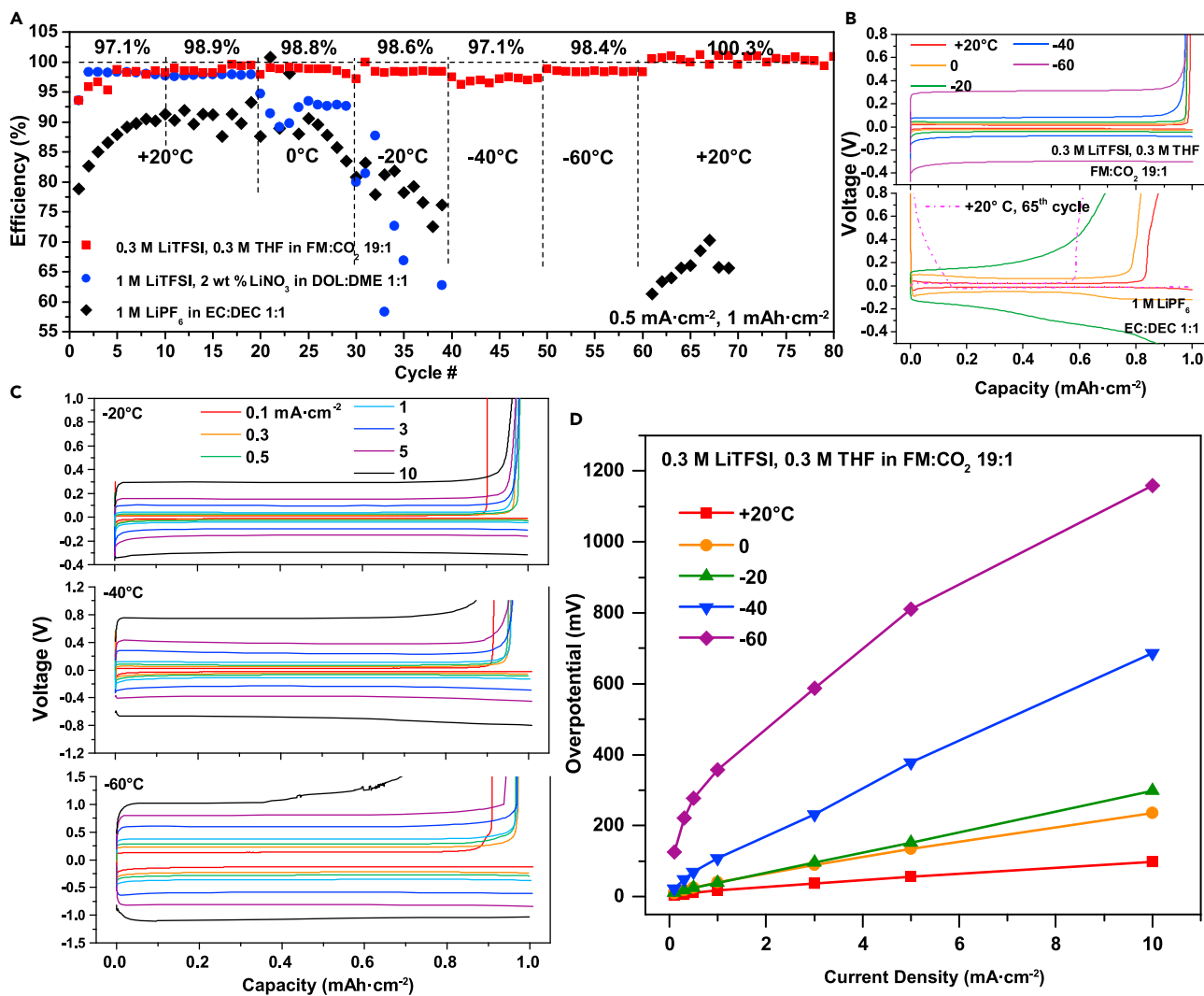
Figure 3. Li-Metal Low-Temperature Electrochemical Performance in Liquefied Gas Electrolyte (corrected)
