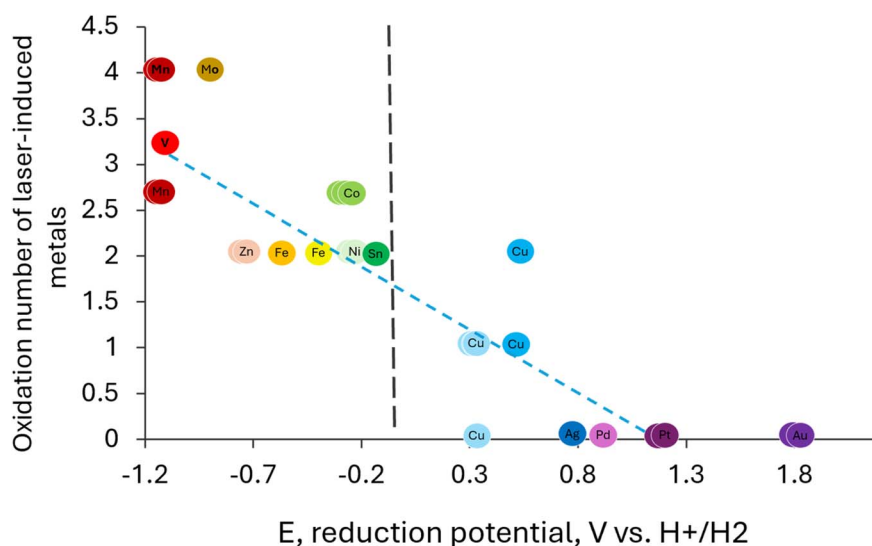
Fig. 1 The oxidation state of laser-induced metals vs. the reduction potential, referring to \text{M}^{x+} + \text{xe}^- \rightarrow \text{M}(\text{s}) . Each color represents a different element. The black line represents the potential of carbon monoxide oxidation. The dashed blue line represents the linear trend. The data and references are presented in Table 1.
