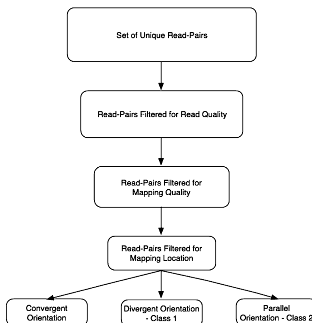
FIG. 1. —Read-pairs included in the analysis were filtered in three ways: 1) Read Quality: Pairs where either read was of all one letter and pairs where the reads were reverse complements of each other were removed. 2) Mapping Quality: At an e value of 10^{-7} both sequences in the read-pair must match exactly once to the genome and must align over all 36 bp with no gaps and up to one mismatch per read. 3) Mapping Location: Both sequences in the read-pair must map to the same chromosome and not to chromosome U or to heterochromatin.
