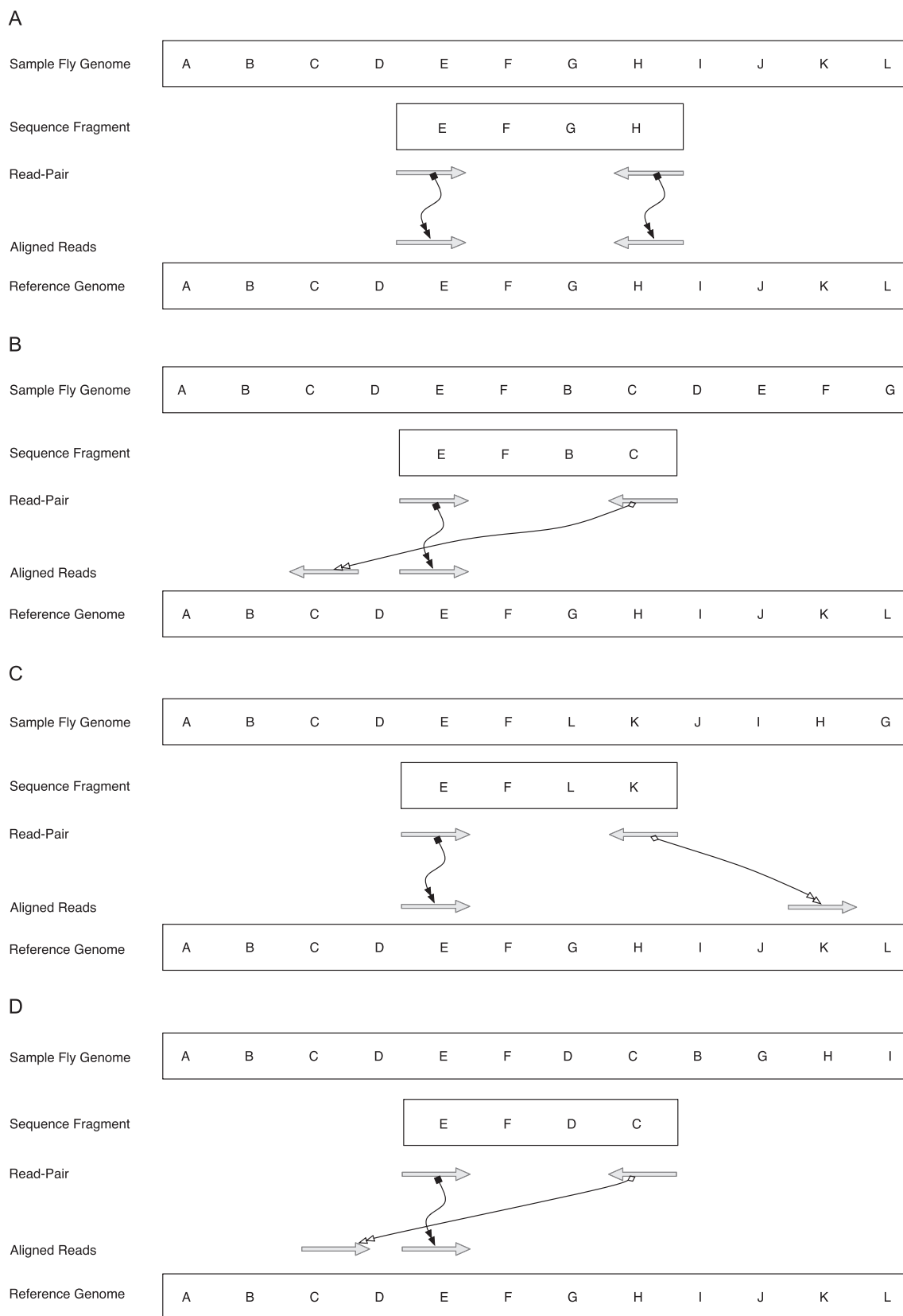
FIG. 2. —Alignment of read-pairs to the reference genome: (A). Expected alignment of read-pairs to the reference genome. (B). Class 1 (tandem duplication). (C). Class 2 (inversion). (D). Class 2 (duplication with a change in orientation).
