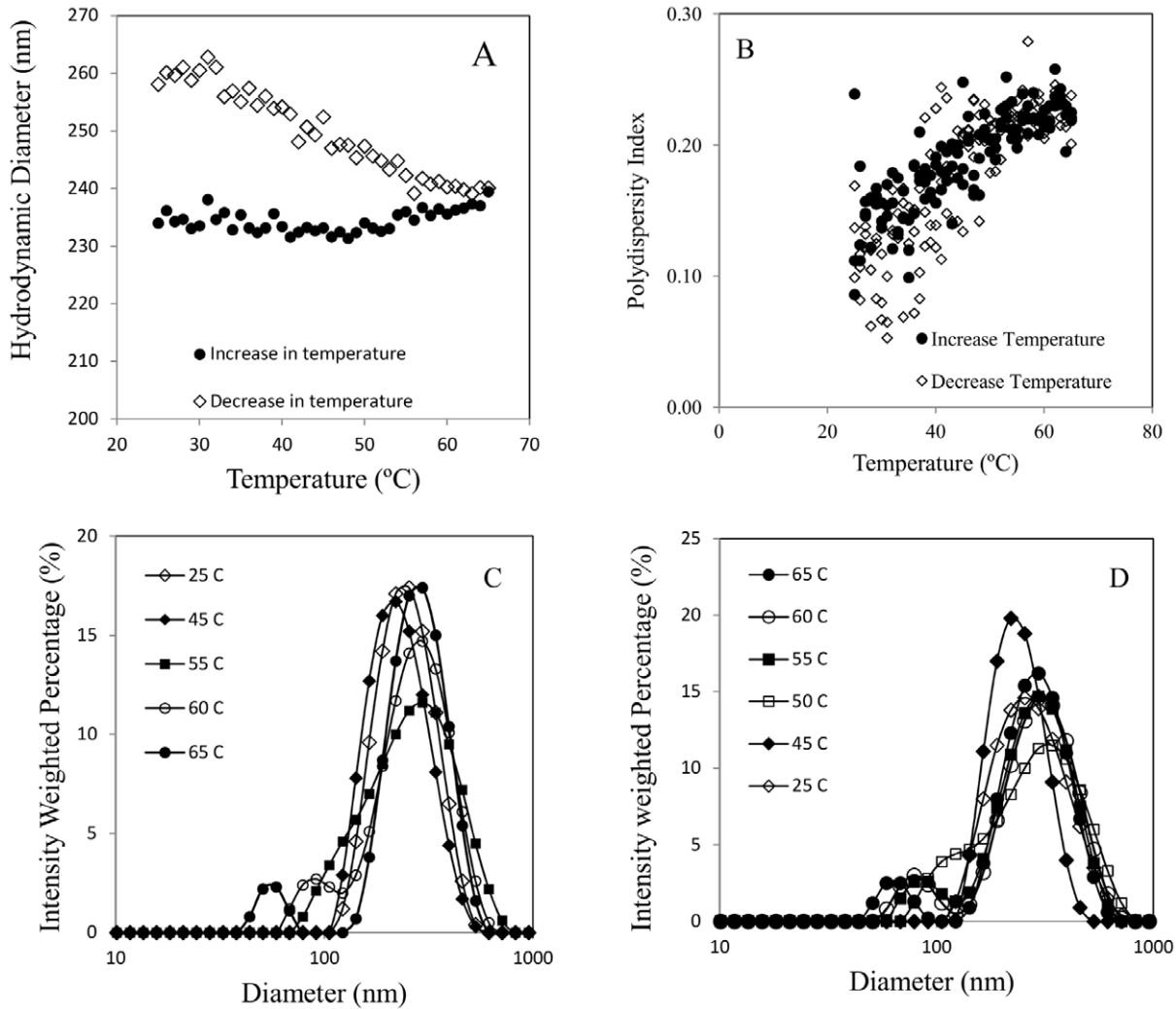
Figure 6. Temperature effect on: (A) hydrodynamic diameter; (B) PDI; (C) intensity weighted size distribution with increasing temperature; (D) intensity weighted size distribution with decreasing temperature. doi:10.1371/journal.pone.0037363.g006
