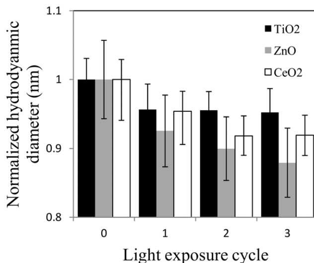
Figure 5. Light induced disagglomeration of metal oxide nanoparticles.
