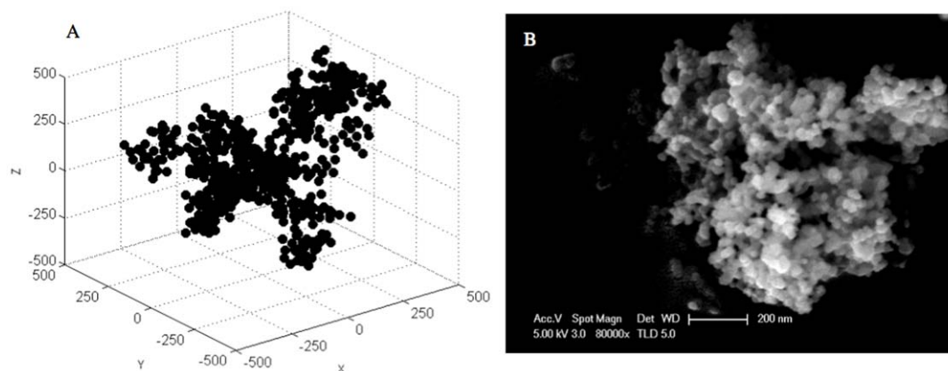
Figure 1. A: A representative aggregate generated by the Matlab code; B: SEM image of a TiO 2 aggregate (Image adapted from Thio, et al. [33], with permission). doi:10.1371/journal.pone.0037363.g001
