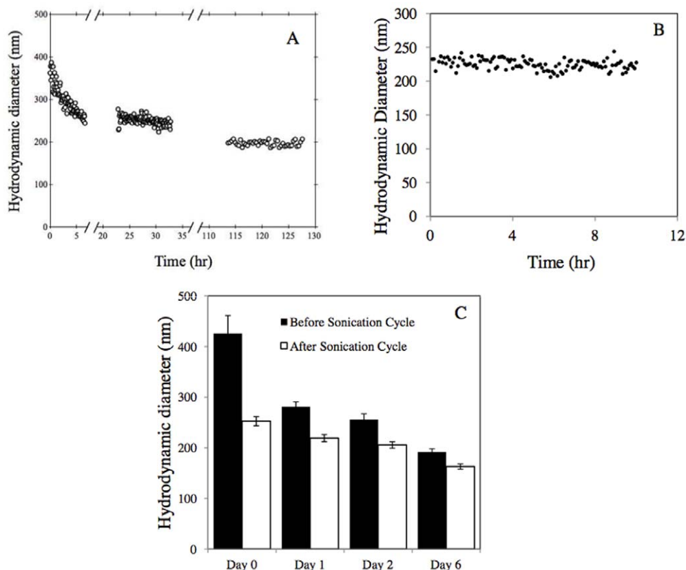
Figure 3. Sedimentation monitored by DLS for (A) TiO 2 agglomerates, prepared by diluting a TiO 2 stock suspension; (B) TiO 2 aggregates, prepared by diluting a TiO 2 stock suspension and sonicating with a sonication probe several times until no further reduction in hydrodynamic size was observed. (C) Hydrodynamic diameter of TiO 2 suspension supernatant monitored for 6 days. doi:10.1371/journal.pone.0037363.g003
