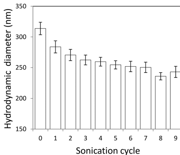
Figure 2. Sonication effect on particle size for a fresh stock of TiO 2 . doi:10.1371/journal.pone.0037363.g002
