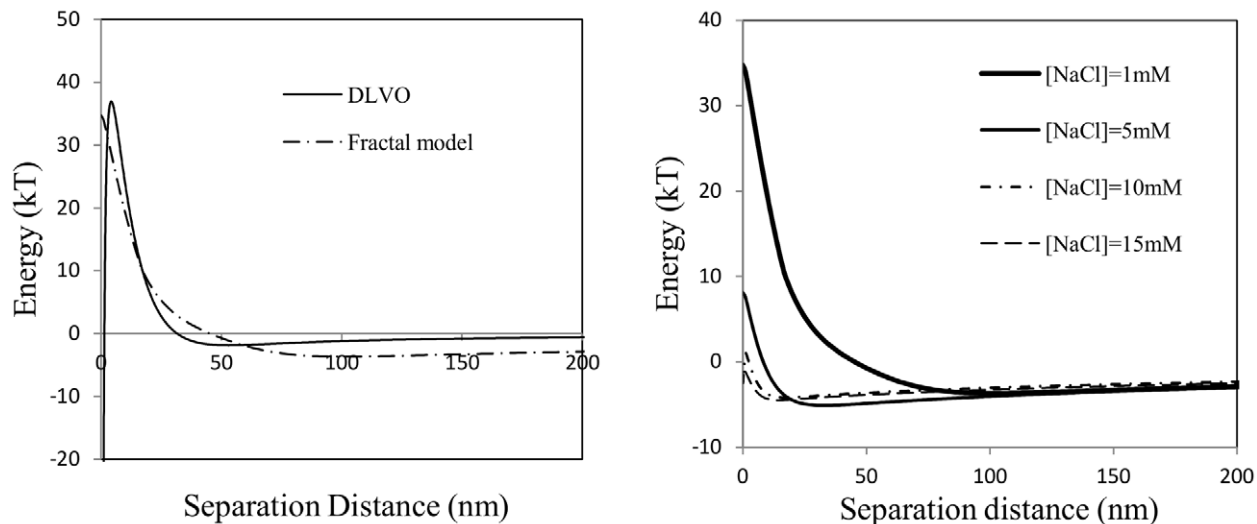
Figure 8. Simulation results considering (A) ionic strength = 0.1 mM; and (B) increasing ionic strength for fractal agglomerates. For particle-particle calculation, d=200 nm. For fractal agglomerates calculation, d_{\text{primary}}=54 nm, 20 primary particles in each aggregate, d_F=1.82 .
