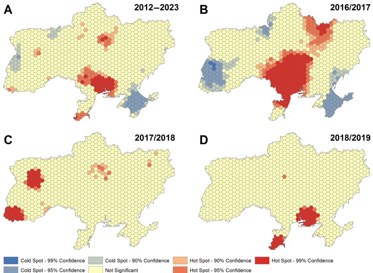
Figure 3. Series of hotspot maps, with colors trending towards red indicating high and trending towards blue low ASF outbreak activity. Panel (A) based on all reported cases from 2012 through May 2023; panels (B–D) by season (April–March) for the years with the highest numbers of ASF outbreaks 2016/2017 (B), 2017/2018 (C) and 2018/2019 (D).
