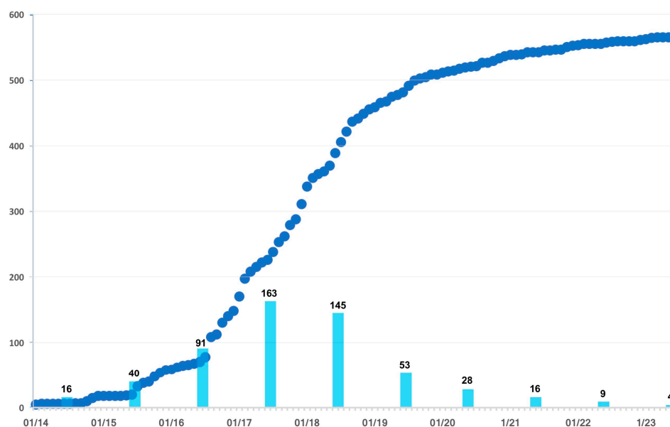
Figure 1. Number of reported ASF cases in Ukraine, depicted on a cumulative monthly basis (dark blue dots) and on a yearly basis (light blue bars) from January 2014 through May 2023.
