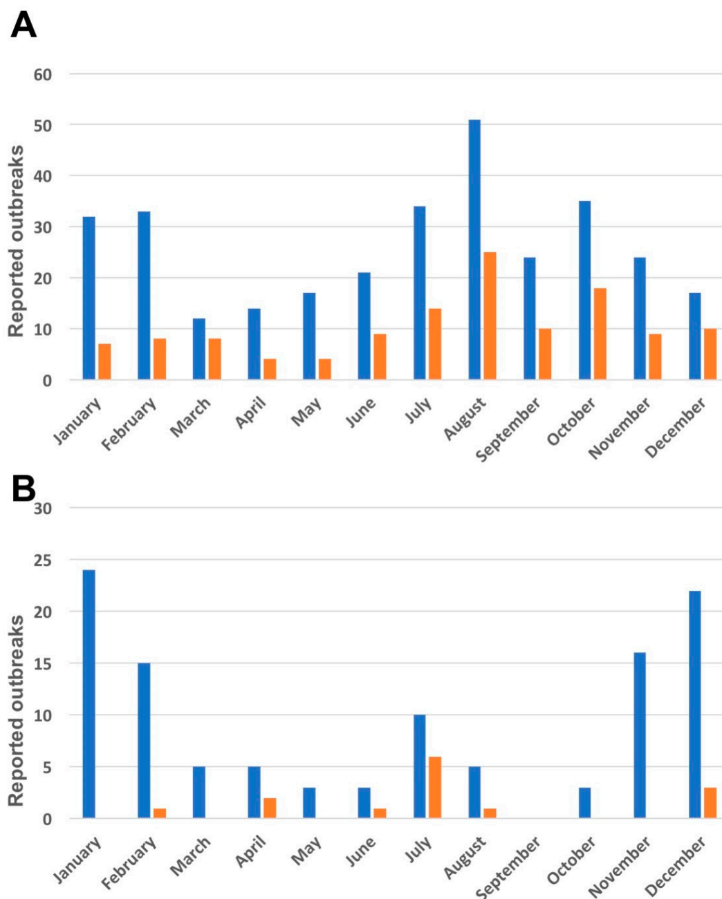
Figure 2. Reported outbreaks by month (cumulative number across all years) broken down by southern (Kherson, Odesa, Mykolaiv; orange bars) and northern (all other; blue bars) oblasts (excluding Crimea); panel (A) showing domestic pig and panel (B) wild boar outbreaks.
