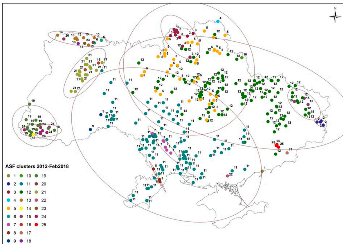
Figure 4. Epidemiological clustering of ASF outbreaks in Ukraine, 2012–2018 (numbered chronologically) according to the “biology and behavioral model”. Ellipses refer to one standard deviation around the mean geographic center of outbreaks.
