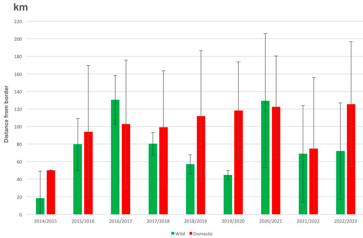
Figure 5. Graph depicting the average distance and standard deviation of outbreaks from official borders or the north of Crimea oblast by season (April–March) for domestic pigs (red) and wild boars (green).
