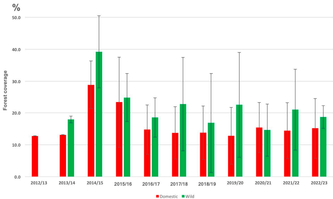
Figure 6. Graph showing the average forest density (circles with a radius of 25 km) around outbreak sites by season (April–March) for domestic pigs (red) and wild boars (green).
