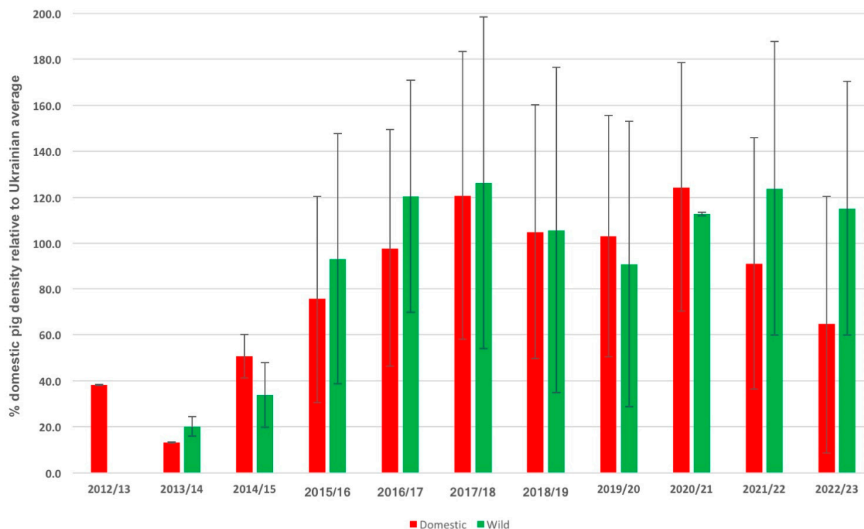
Figure 7. Graph showing the correlation between outbreaks in domestic pigs (red) and wild boars (green) with the modelled population density of domestic pigs in Ukraine in the surrounding area (circles with 25 km radius). Data by season (April–March) and displayed in % of average pig density in Ukraine with standard deviations.
