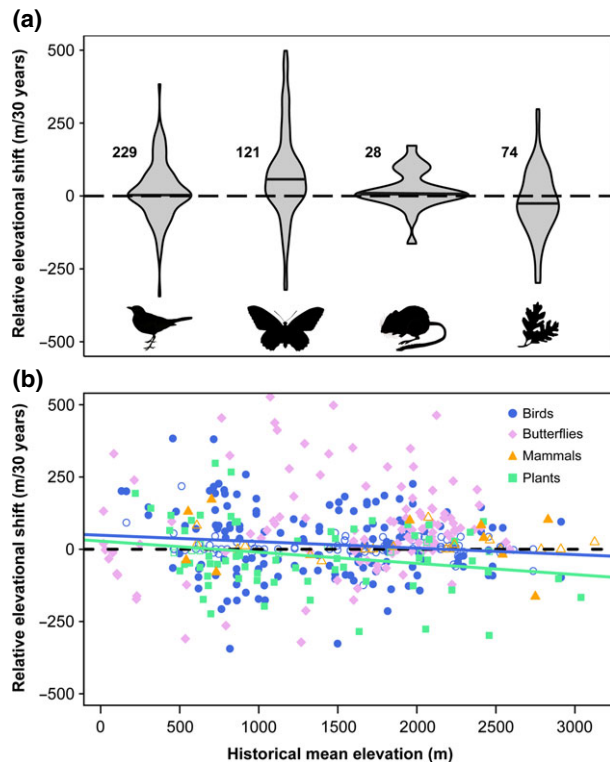
Fig. 3 Relative elevational shifts during the 20th century from published studies of birds (Tingley et al. , 2012), butterflies (Forister et al. , 2010), mammals (Moritz et al. , 2008) and plants (Kelly & Goulden, 2008; Crimmins et al. , 2011) in California. Estimates of elevational shift and historical elevation (either as a mean or an optimum) were derived from individual studies. Relative shifts in elevational range across the four groups are calculated relative to the shortest study time period (30 years; Kelly & Goulden, 2008). Analysis was limited to relative shifts between -500 and 500 m per 30 years, which excluded 7 (5%) butterfly populations that shifted >500 m per 30 years. (a) Violin plot of relative elevational shift ( \text{m yr}^{-1} ) for the four taxonomic groups. Violins are scaled to have the same area across the four groups. Numbers adjacent to violins indicate the number of individual population shifts for each group. Bold horizontal lines represent the median relative elevational shift for each group. (b) Scatter plot of relative elevational shift ( \text{m yr}^{-1} ) against mean historical elevation (m) for the four taxonomic groups. Closed symbols refer to significant shifts and open symbols refer to nonsignificant shifts, as assessed by the individual studies. Trend lines illustrate the results of the two significant linear models of relative elevational shift as a function of historical elevation: birds (slope = -0.022 , t_{227} = -2.216 , P < 0.05 ) and plants (slope = -0.039 , t_{72} = -2.098 , P < 0.05 ). Data on mammals, birds, and historical occurrence of most plants included in this figure can be accessed via http://ecoengine.berkeley.edu . All icons were obtained from the Integration and Application Network at the University of Maryland Center for Environmental Science ( www.ian.umces.edu/imagelibrary ).
