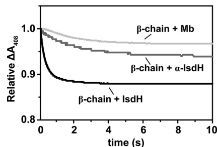
Figure 4. Hemin transfer from isolated \beta -globin chains. Representative stopped-flow time courses show absorbance changes at 408 nm ( \Delta A_{408} ) after mixing 5 \mu M isolated Met \beta -globin chains with 150 \mu M apo-receptor or 50 \mu M apo-Mb. Relative spectral traces are shown for comparison in which all starting absorbances were normalized to a value of 1. Only the first 10 s are shown as absorbance artifacts were observed after this time as a result of the slow process of apo-globin denaturation.
