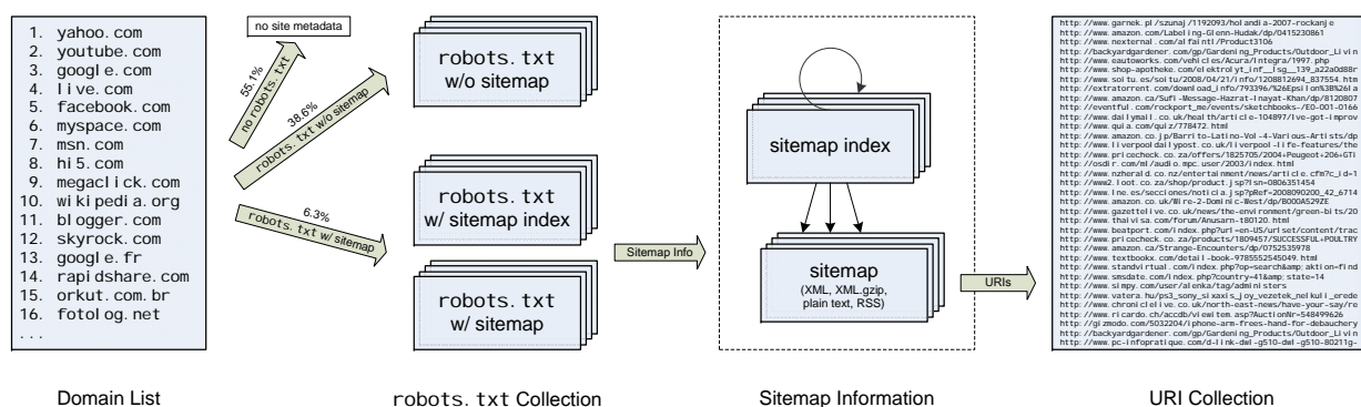
Figure 8: Overview of the Crawling Process
