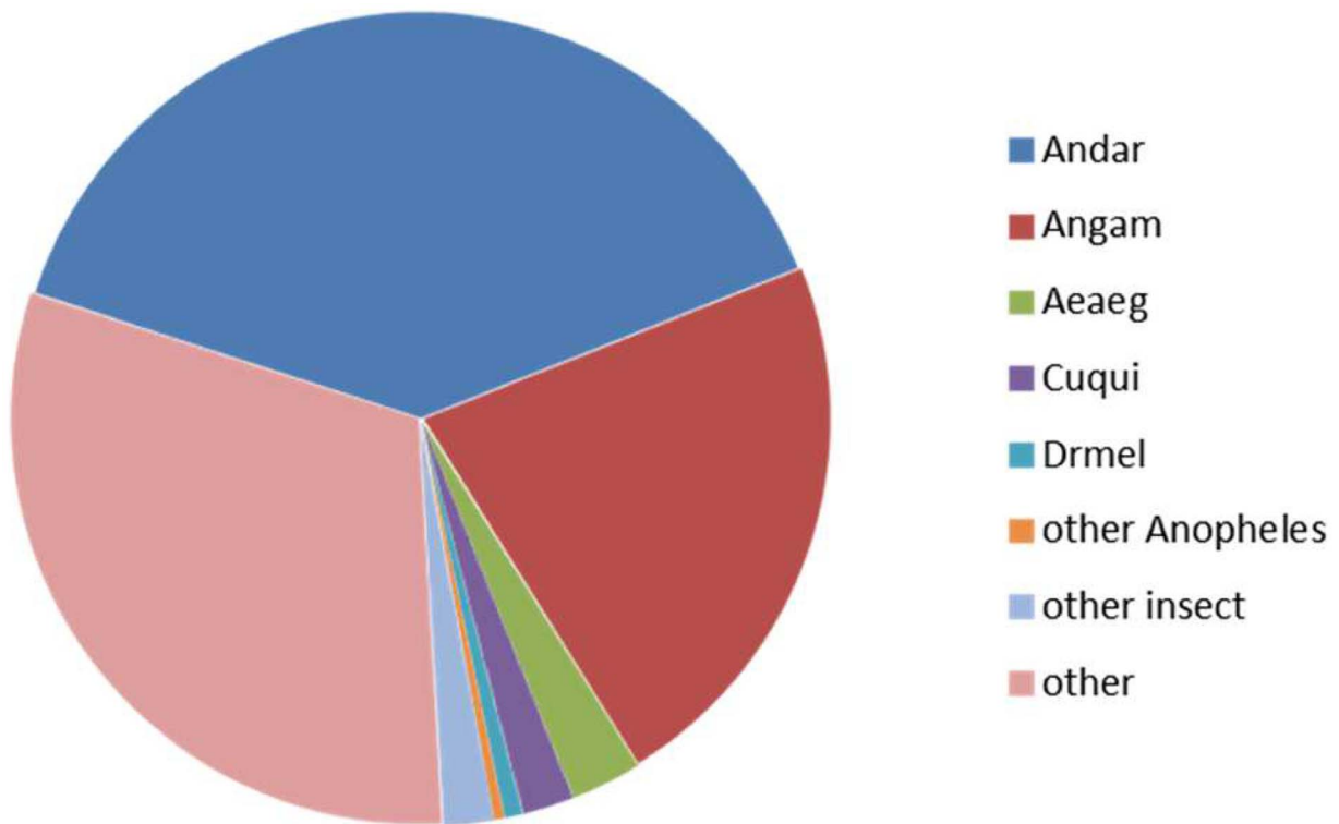
Figure 2. Distribution of the best matches of all An. aquasalis predicted proteins by organisms: Andar- An. darlingi ; Angam- An. gambiae ; Aeaeg, Ae. aegypti ; Cuqui, Cu. quinquefasciatus ; Drmel, D. melanogaster ; Other Anopheles species; Other insects- not of the Anopheles genus; Other- non-insect organisms. doi:10.1371/journal.pntd.0003005.g002
