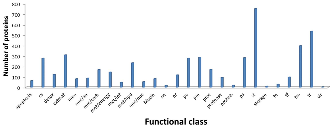
Figure 3. Classification of the annotated An. aquasalis proteins in functional categories. The numbers in parenthesis indicate the number of proteins in each category. apoptosis (64), cs- Cytoskeletal (278), detox- Detoxification (123), extrmat- Extracellular matrix and adhesion (310), imm- Immunity (81), met/aa- Amino acids metabolism (145), met/carb- Carbohydrate metabolism (169), met/energy- Energy metabolism (145), met/int- Intermediary metabolism (48), met/lipid- Lipid metabolism (234), met/nuc- Nucleotide metabolism (54), mucin (82), ne- Nuclear export (19), nr- Nuclear regulation (118), pe- Protein export machinery (278), pm- Protein modification machinery (287), prot- Proteasome machinery (170), protease (94), protinh- Protease inhibitor (20), ps- Protein synthesis (283), st- Signal transduction (752), storage (11), te- Transposable element (29), tf- Transcription factor (97), tm- Transcription machinery (397), tr- Transporters and storage (536), vir- Viral product (4). doi:10.1371/journal.pntd.0003005.g003
