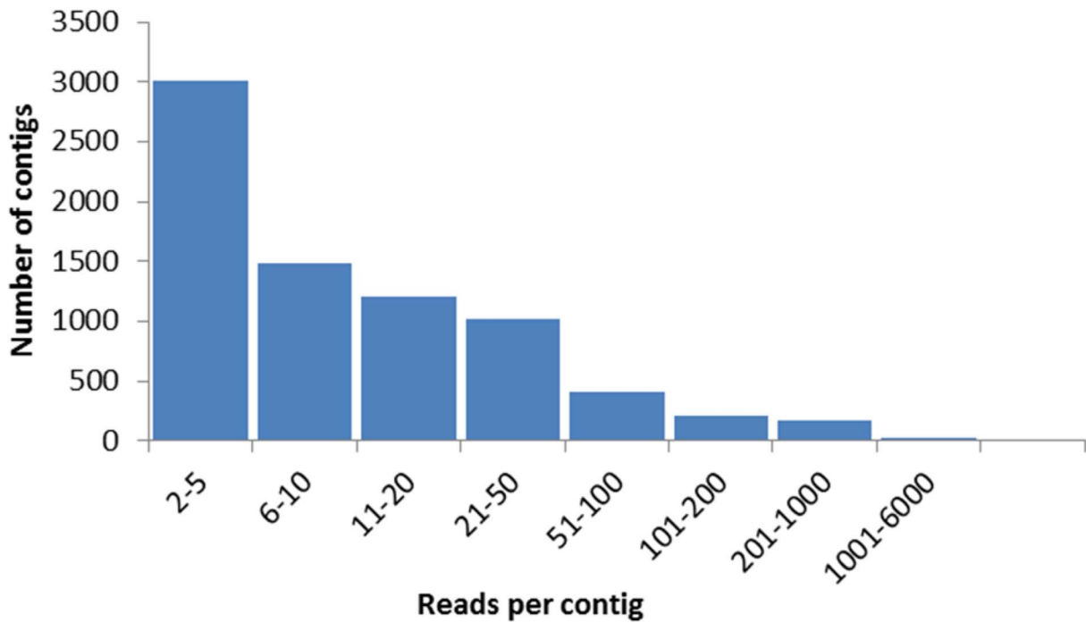
Figure 1. Number of sequences composing the assembled An. aquasalis contigs. A total of 7544 contigs were assembled from \geq 2 sequences. The number of sequences that compose each contig varies from 2 to 5,207, with an average of 35 sequences per contig. Forty-three percent of the assembled contigs contained 10 or more sequences. doi:10.1371/journal.pntd.0003005.g001
