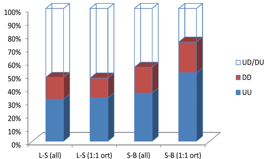
Figure 4. Comparisons of developmental changes in gene expression between An. aquasalis and An. gambiae . Developmental gene regulations [up(U) or down(D)-regulation] between larvae and sugar fed females (L-S all) or between sugar fed females and blood fed females (S-B all) of An. aquasalis transcripts that have a homolog An. gambiae (best Blast match) represented in the GeneChip Plasmodium/Anopheles Genome Array [42,95] were compared. The pairwise comparisons including all An. aquasalis/An. gambiae homologous pairs of genes demonstrated a lack of conservation of developmental changes in transcript abundance between the two mosquito species. Similar analyses restricting the transcript list to putative 1:1 ortholog pairs, defined by reciprocal blast and only those significantly regulated in An. aquasalis , with at least 3 fold change between two compared samples (L-S 1:1 ort or S-B 1:1 ort) showed that 75% the transcripts regulated by blood feeding were consistently up or down regulated in both species. Using the same restricted list of transcripts, only 49% of the transcripts were consistently up- or down-regulated between L-S in both species. Genes up-regulated or down-regulated in both species are indicated by (UU) or (DD), respectively. Transcripts differentially regulated between the two species are indicated by (UD/DU). doi:10.1371/journal.pntd.0003005.g004
