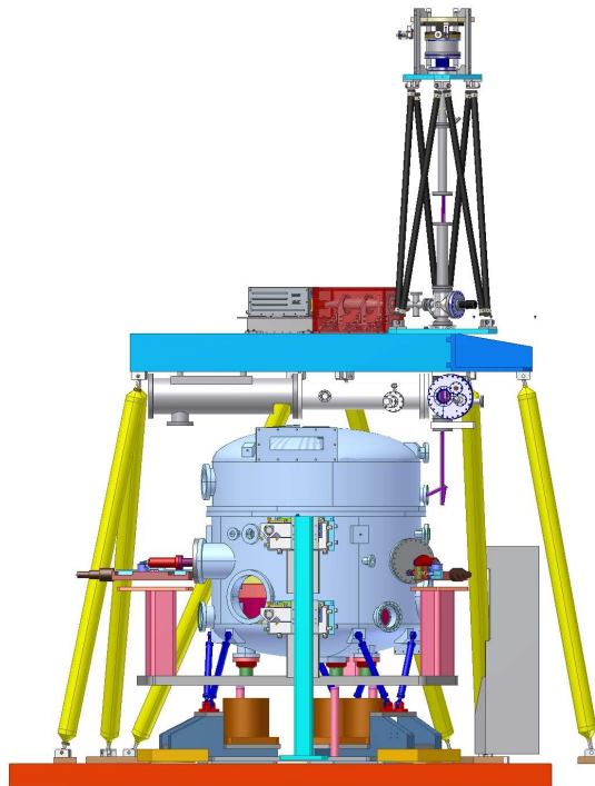
Figure 13: Proposed design for DUV/UV source input to MET
