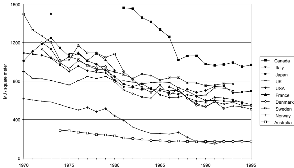
Figure 20. Fuel Use per Commercial Buildings Floor Area in Selected Industrialized Countries, 1970-1995. Reference: Krackeler et al., 1998.
