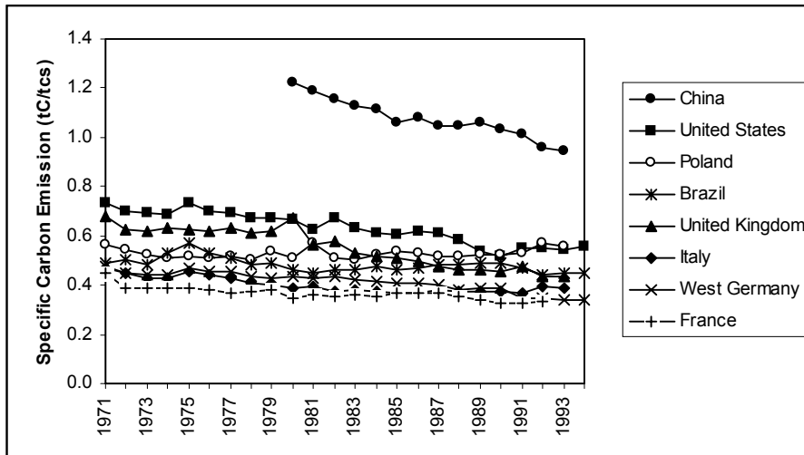
Figure 21. Trends in Specific Carbon Emissions for the Production of Crude Steel in Major Steel Producing Countries, 1971-1994 (expressed in tonne C/tonne crude steel). References: Worrell et al., 1997b; Faaij et al., 1995.
