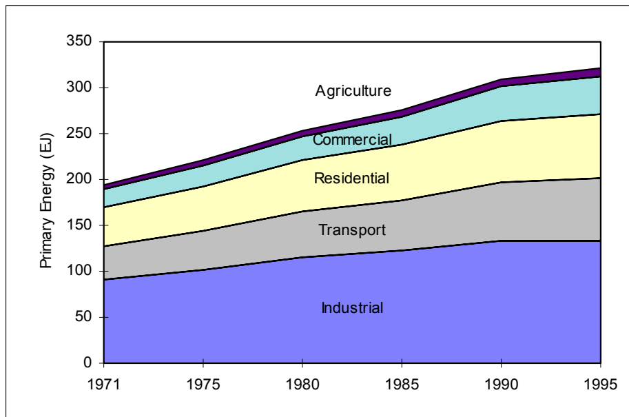
Figure 1. Global Primary Energy Use by Sector, 1971 to 1995.
