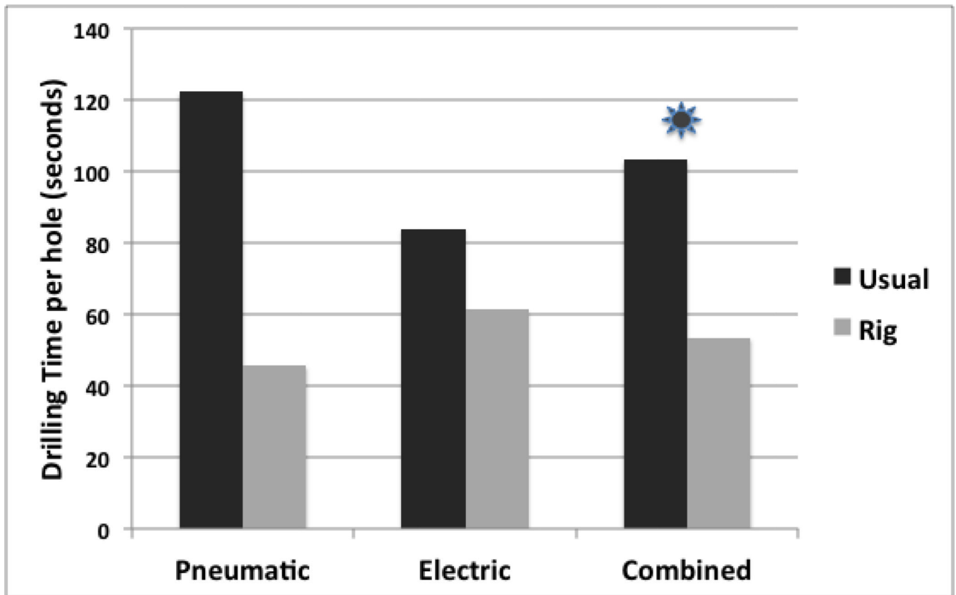
FIGURE 6. Productivity: mean drilling time per hole comparing the usual method to drilling with the universal rig during identical drilling conditions in the field. When combined (N=6), productivity was significantly better ( p=0.03 ) with the rig when compared to the usual method.
