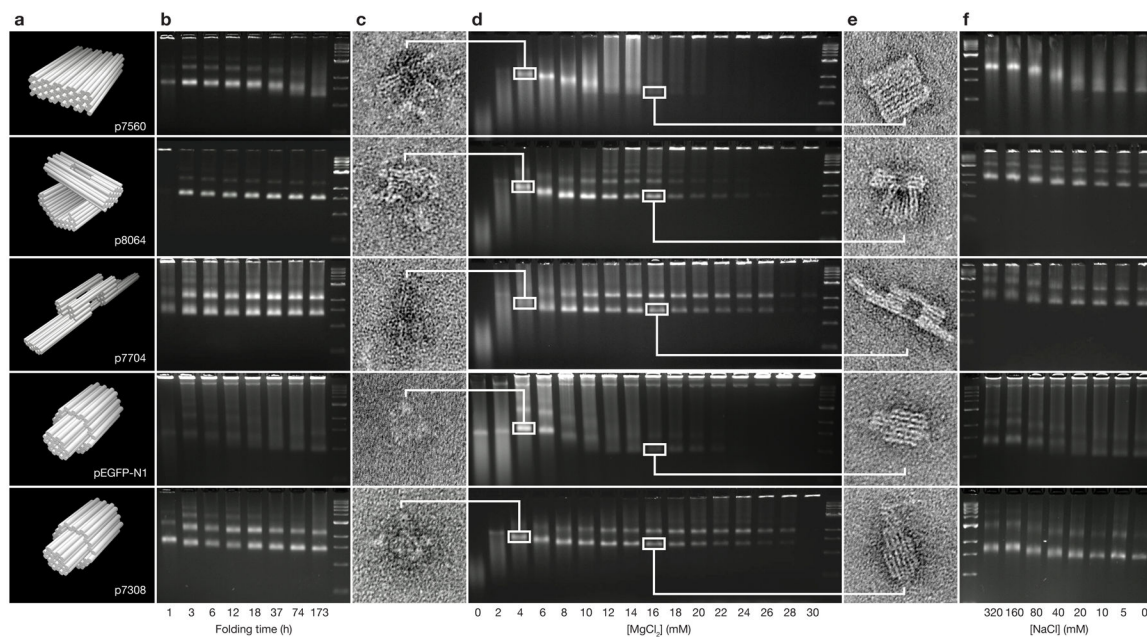
Figure 3. Gel and TEM analysis of folding conditions for three-dimensional DNA origami a , Cylinder models of shapes: monolith, stacked cross, railed bridge, and two versions of genie bottle, with corresponding scaffold sequences. b , Shapes were folded using different thermal-annealing ramps (1.2 h: 95°C to 20°C at 1.6 min/°C; 3 h, 6 h, 12 h, 18 h, 37 h, 74 h, 173 h: 80°C to 60°C at 4 min/°C, followed by 60°C to 24°C at 5, 10, 20, 30, 60, 120, or 280 min/°C, respectively) in 5 mM Tris, 1 mM EDTA, and 16 mM MgCl 2 and analyzed by gel electrophoresis (2% agarose, 0.5 × TBE, 11 mM MgCl 2 ). c–e , TEM and gel analysis of influence of MgCl 2 concentration on folding quality. c , The fastest-migrating bands in the 4 mM MgCl 2 lanes were purified and imaged, revealing gross folding defects. d , Shapes were folded with a 173 h ramp in 5 mM Tris, 1 mM EDTA, and MgCl 2 concentrations varying from 0 to 30 mM. e , As in c , leading bands were purified from the 16 mM MgCl 2 lanes and found to exhibit higher-quality folding when analyzed by TEM. f , Excess NaCl inhibits proper folding. Shapes were folded with 173 h ramp in 5 mM Tris, 1 mM EDTA, 16 mM MgCl 2 , and varying NaCl concentrations.
