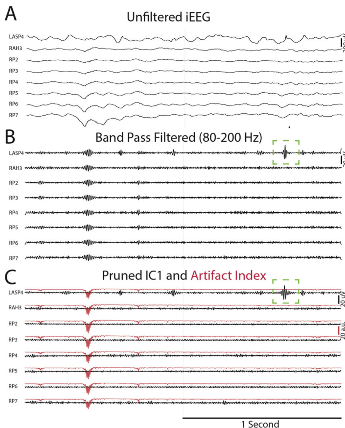
Fig. 2. Illustration of the utilization of independent component analysis (ICA) for artifact reduction, rejection of artefactual ripples, and improvement in ripple signal to noise. An iEEG recording from eight contacts in referential montage (A) demonstrates no obvious artifact. Band-pass (80–200 Hz) filtering (B) reveals a ripple occurring synchronously in all the recordings, follow by a ripple with an unconvincing morphology in LASP4 (green box). Performing ICA on the band-pass filtered signal and pruning independent component 1 (C) results in the elimination of the first ripple in all the recordings, and the unmasking of additional oscillatory cycles in the subsequent ripple in LASP4 (green box). The artifact index (red) indicates the epoch in which the artefactual HFO contaminated the recording. (For interpretation of the references to color in this figure legend, the reader is referred to the web version of this article.)
