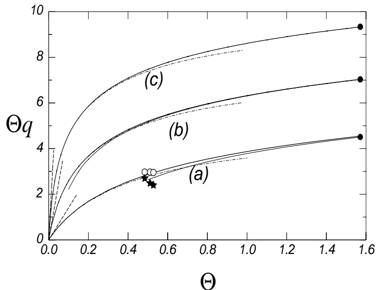
FIGURE 3. Heat flow q = q_*/(K\Delta T) as a function of \Theta and \mathcal{B} = ha/K . Curves, conduction model for (a) \mathcal{B} = 40 , (b) 500, (c) 5000: heavy curves, composite expansion (13); light curves, fixed- \Theta expansion (7); broken curves, small- \Theta expansion (11); broken lines, small- \Theta limit (35); \bullet , equation (A 5). Symbols, free-boundary problem: \circ , equation (33); \star , Schonberg et al (1995).
