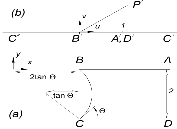
FIGURE 4. The conformal mapping used to solve (3).
