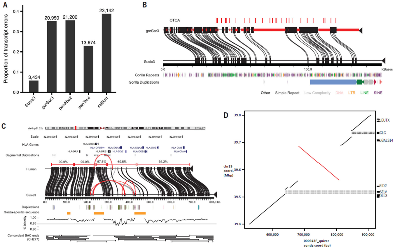
Fig. 4. Gene annotation and structural variation
