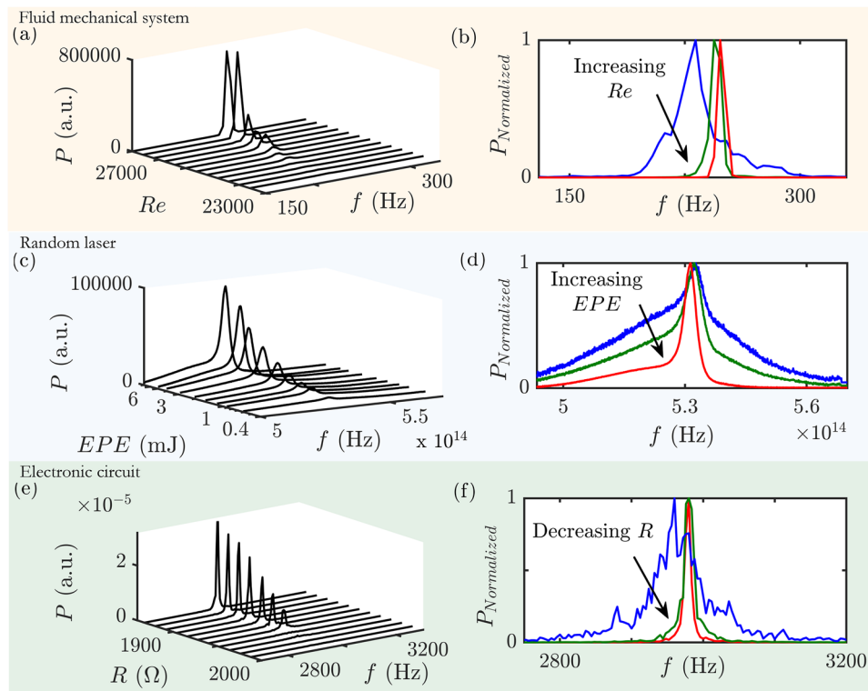
Figure 2. Evolution of the spectrum for fluid mechanical, optical and electronic systems. The evolution of power spectrum with variation in the corresponding control parameter is presented on the left side and the normalized spectra for each system are given on the right side of the panel. (a,b) Power spectra obtained using Fast Fourier Transform (FFT) of the acoustic pressure fluctuations for a laboratory-scale bluff body stabilized combustor of length 700 mm. The power spectra exhibit an increasing dominance of a single peak on approaching oscillatory instabilities (for increasing Re ) in all the fluid mechanical systems discussed in this paper, and hence this figure is a representative example. (c,d) Emission spectra of the random laser as we progressively increase EPE. The power spectrum is obtained by multiplying the photon count per second for each wavelength with its respective energy. The broad spectrum starts to become a narrow lasing-like peak with increase in EPE. (e,f) Power spectra obtained using FFT of the voltage signal ( v_1 ) measured from Chua’s circuit and the corresponding normalized spectra are shown respectively. The peak sharpens during the transition to limit cycle oscillations as the resistance ( R ) is decreased. The power spectra using FFT are plotted for a resolution of 4 Hz for visualization purpose.
