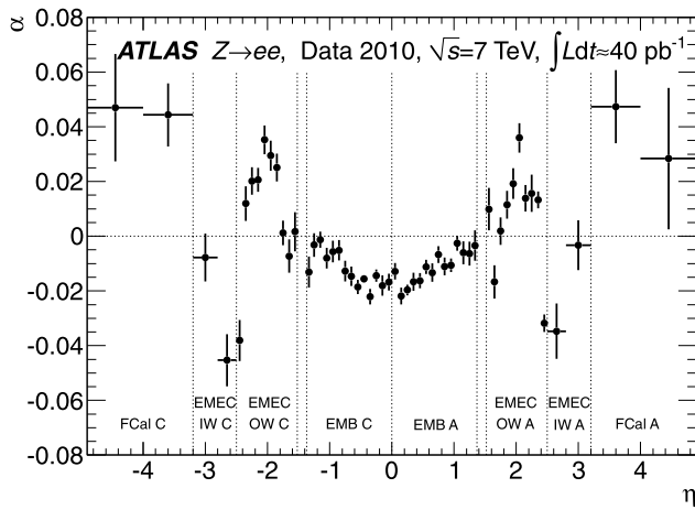
Fig. 4 The energy-scale correction factor \alpha as a function of the pseudorapidity of the electron cluster derived from fits ( left ) to Z \rightarrow ee data and ( right ) to J/\psi \rightarrow ee data. The uncertainties of the Z \rightarrow ee measurement are statistical only. The J/\psi \rightarrow ee measurement was made
