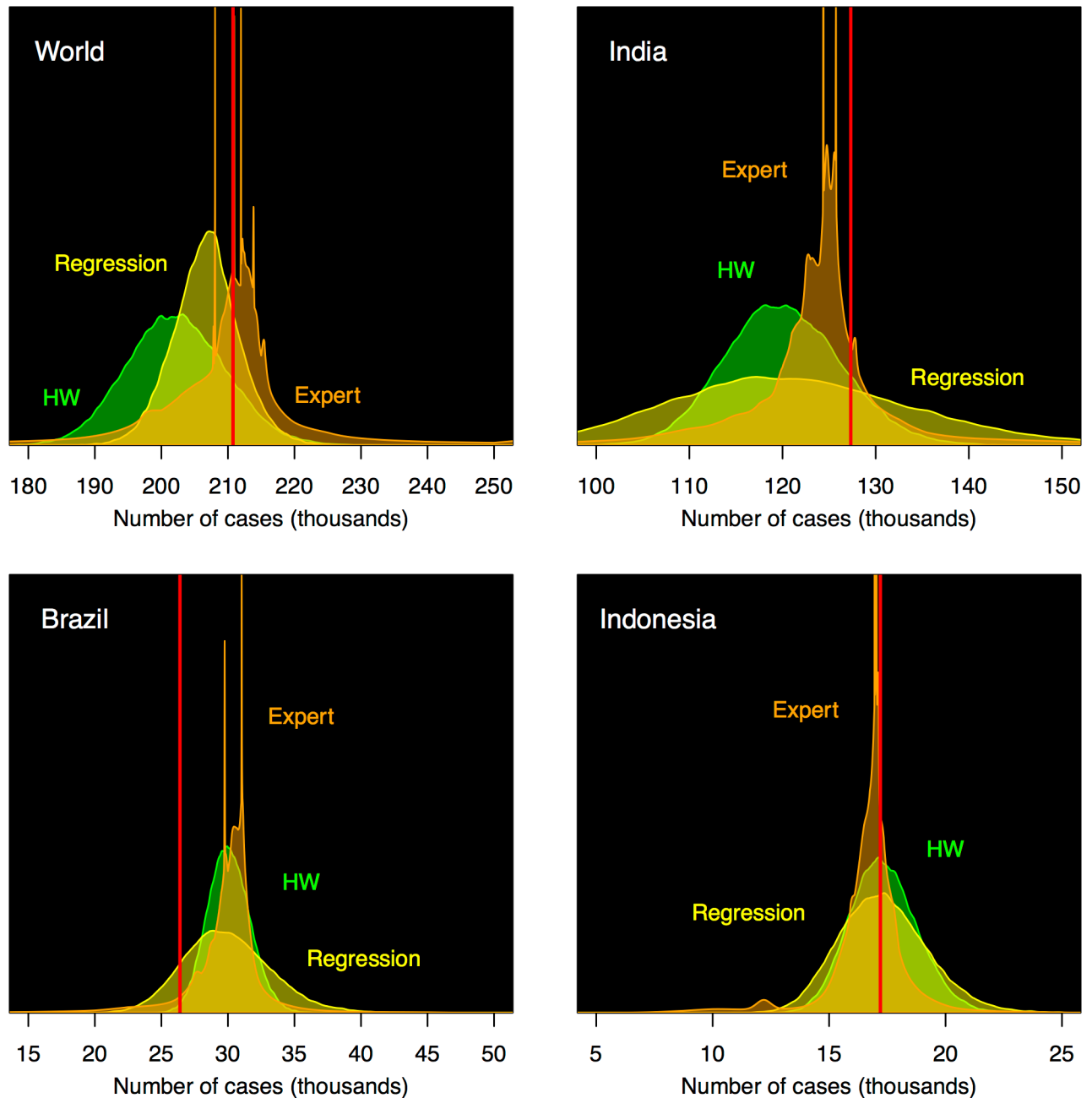
Fig 2. Probabilistic forecasts for the distribution of leprosy cases for the year 2015 for the world, India, Brazil, and Indonesia, derived from experts (orange), regression (yellow), and simple Holt-Winters (green). The vertical axis shows density; the red line indicates where the observed data fell.
