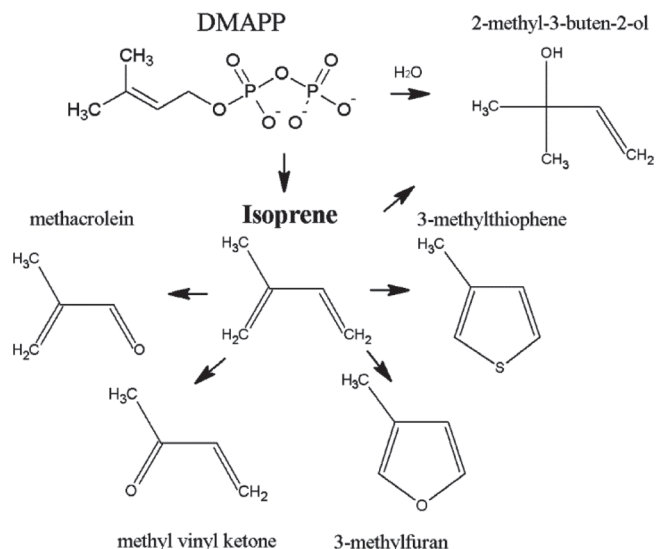
Fig. 1. Diagram of isoprene and its potential oxidation products. Isoprene is first synthesized from dimethylallyl diphosphate (DMAPP), which might also form MBO if water is allowed to enter the active site of isoprene synthase (Gray et al. , 2011). Isoprene may then be oxidized to MACR, MVK, 3-MF, 3-MT, and MBO via enzymatic and/or non-enzymatic mechanisms.
