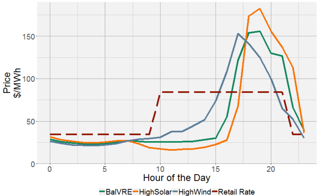
Figure 23. A low VRE two-period TOU rate in NYISO compared to high VRE prices
