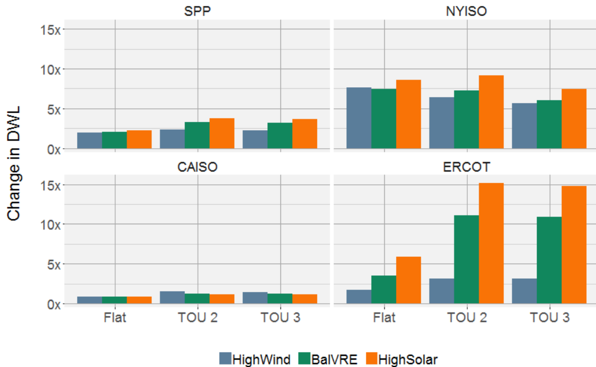
Figure 24. Economic performance of low VRE rates in a high VRE scenario
