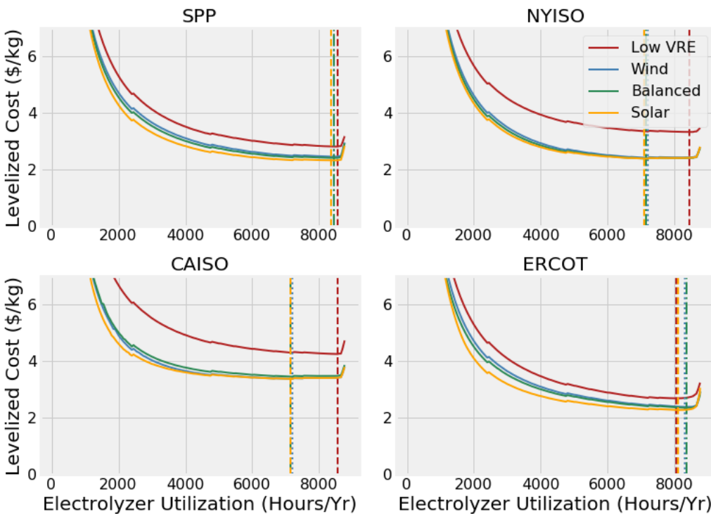
Figure B-4. Cost minimizing utilization rates of the electrolyzer at $900/kW (1500 fully burdened)
