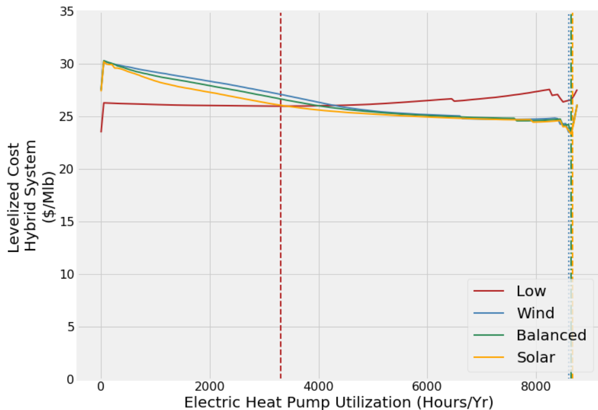
Figure B-11. Optimal heat pump utilization rates in a hybrid setting in ConEd’s Manhattan DE system
