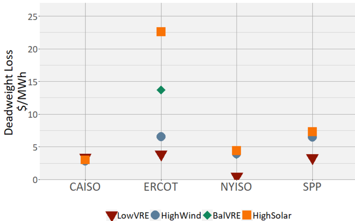
Figure 22. Economic performance of a flat rate structure in low VRE and high VRE scenarios
