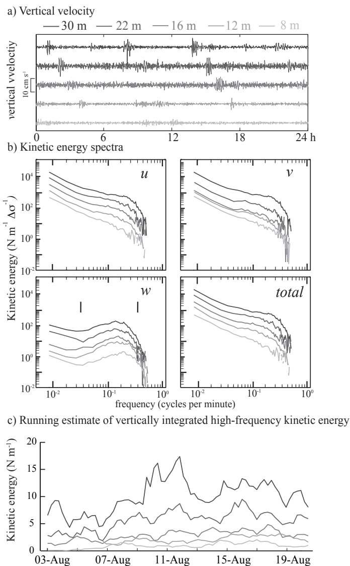
Figure 2.9: Panel a: 24 h time series of vertical velocity across the ADCP array (18-August-2006). Packets of high-frequency internal waves arrived twice daily, and were observed to propagate coherently across the array, decreasing in magnitude in shallower waters. Panel b: Vertically integrated kinetic energy spectra of cross-shore ( u ), along-shore ( v ), and vertical velocity ( w ). The vertical bars on the w panel represent the high-frequency internal wave band. The elevated shoulder of energy was associated with the passage of high-frequency internal waves. Panel (c): Running estimates of frequency and vertically integrated high-frequency total kinetic energy. High-frequency kinetic energy variability peaked between 10-August and 12-August, in concert with the peak internal tide energy.
