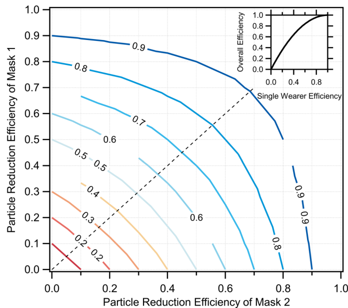
Figure 7. The net particle reduction efficiency with masks worn by source persons and receptor persons, for the wearer masks having varying efficiency. (Inset) The overall reduction efficiency versus single mask reduction efficiency assuming the same mask efficiency for the source person and receptor person.
