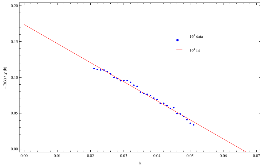
Figure 10: Inverse of the logarithmic derivative of the average curvature \mathcal{R}(k) [defined in Eq. (82)] on the 16^4 lattice with with 65, 536 sites. The straight line represents a best fit of the form A(k_c - k) for k \geq 0.02 . The location of the critical point in k is consistent with the earlier estimate coming from the average curvature \mathcal{R}(k) and its fluctuation \chi_{\mathcal{R}}(k) . From the slope of the line one then computes directly the exponent \nu .
