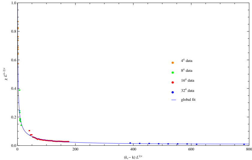
Figure 14: Finite size scaling behavior of the scaled curvature fluctuation \chi_{\mathcal{R}}(k, L) \cdot L^{4-2/\nu} versus the scaled coupling (k_c - k) \cdot L^{1/\nu} . Here L = 4, 8, 16, 32 for a lattice with L^4 sites. The continuous line represents a best fit to a scaling function of the form 1/(a + b x^c) , and finite size scaling predicts that all points should lie on the same universal curve. The continuous line corresponds to a critical point k_c = 0.06384(40) and an exponent \nu = 0.3389(56) .
