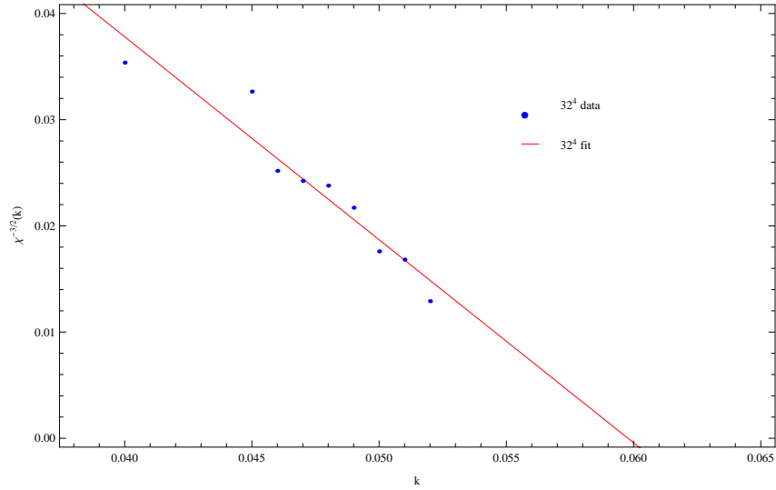
Figure 9: Inverse curvature fluctuation raised to the power 3/2 , on the 32^4 lattice; note that the data is scaled by a factor of \times 100 . The straight line represents a linear fit of the form A(k_c - k) . The location of the critical point in k is consistent with the estimate obtained from the average curvature on the same size lattice, here with a larger uncertainty.
