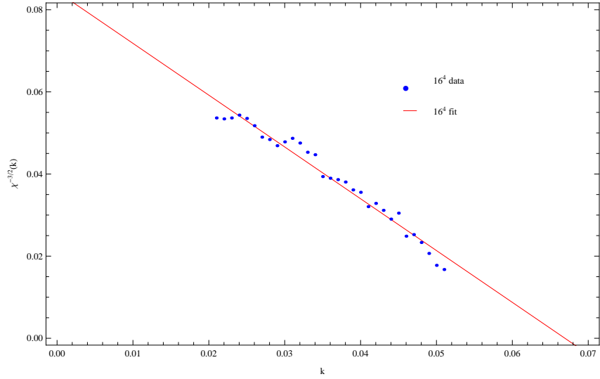
Figure 8: Inverse curvature fluctuation raised to the power 3/2 , on the 16^4 lattice; note that the data is scaled by a factor of \times 100 . The straight line represents a linear fit of the form A(k_c - k) . The location of the critical point in k is consistent with the estimate obtained from the average curvature, but with a somewhat larger error.
