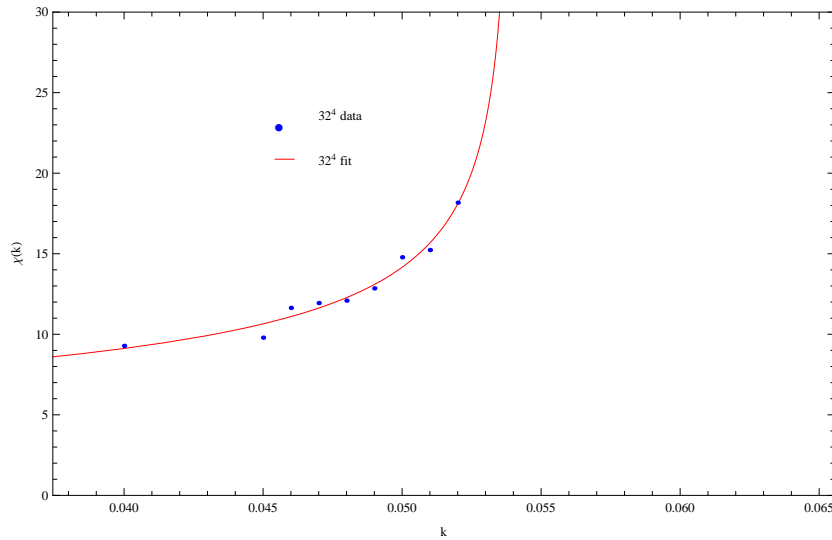
Figure 7: Curvature fluctuation \chi_{\mathcal{R}}(k) on the 32^4 lattice with 1,048,576 sites. Note the change in scale from the previous figure. The line shown is a best fit of the form \chi_{\mathcal{R}}(k) = A(k_c - k)^{-(1-\delta)} for k \geq 0.04 .
