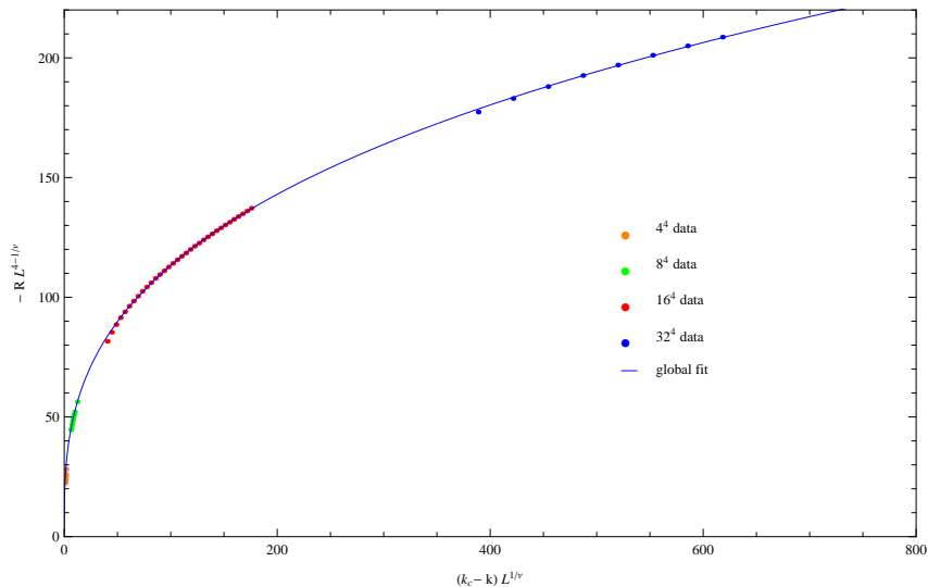
Figure 13: Finite size scaling behavior of the scaled curvature \mathcal{R}(k, L) \cdot L^{4-1/\nu} versus the scaled coupling (k_c - k) \cdot L^{1/\nu} . Here L = 4, 8, 16, 32 for the lattice with L^4 sites. Statistical errors are comparable to the size of the dots. The continuous line represents a best fit to a scaling function of the form a + b x^c , and finite size scaling predicts that all points should lie on the same universal curve. The continuous line corresponds to a critical point k_c = 0.06388(32) and exponent \nu = 0.3334(4) .
