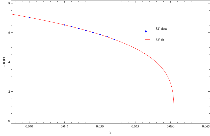
Figure 2: Average local curvature \mathcal{R}(k) as defined in Eq. (14), computed on a large lattice with 32^4 = 1,048,576 sites. Note the change in horizontal scale as compared to the previous figure. Statistical errors ( \sim \mathcal{O}(10^{-4}) ) are much smaller than the size of the symbols. The continuous line represents a fit of the form A (k_c - k)^\delta for k \geq 0.04 , with exponent \delta = 4\nu - 1 .
