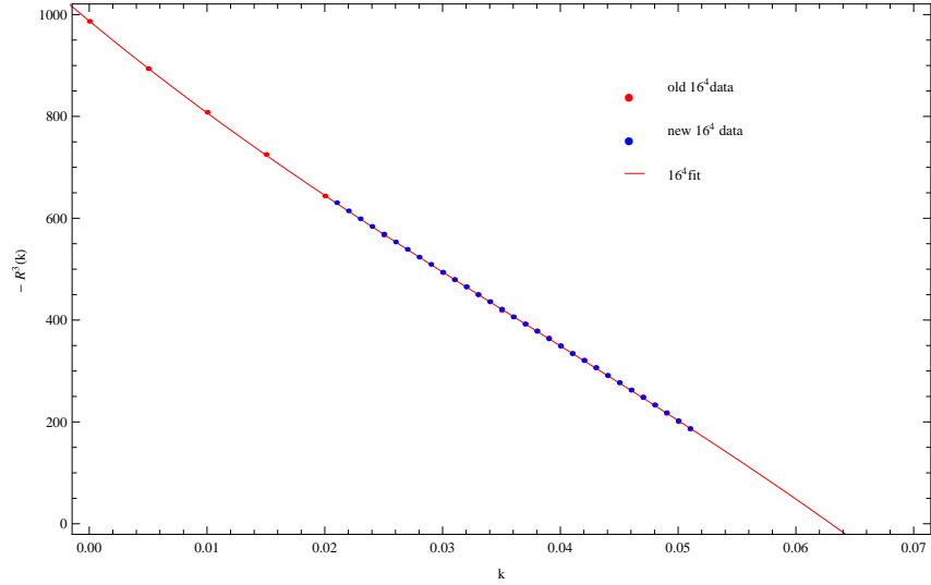
Figure 3: Average local curvature \mathcal{R}(k) on the 16^4 lattice, raised to the third power. If \delta = \nu = 1/3 exactly, then all the data should fall on a straight line close to k_c . The continuous line here represents a linear fit of the form A (k_c - k) for k \geq 0.02 . Deviations from linearity of the transformed data are rather small.
