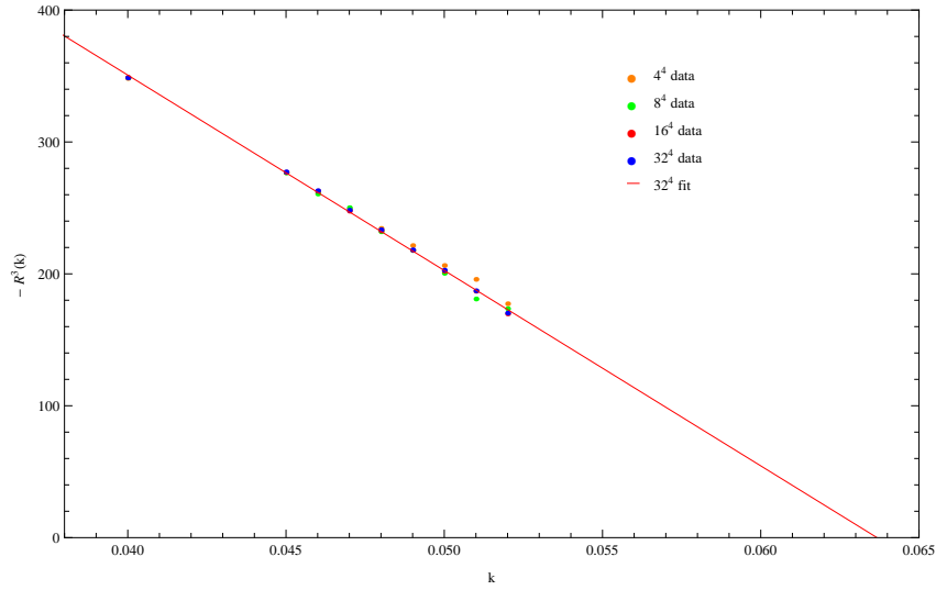
Figure 5: Volume dependence of the average local curvature |\mathcal{R}(k)|^3 on lattices with 4^4 , 8^4 , 16^4 and 32^4 sites. Again, if \delta = \nu = 1/3 exactly, then the data should all fall on a straight line close to k_c . The continuous line represents a linear fit of the form A(k_c - k) . The size dependence becomes rather small on the larger lattices, unless one moves very close to the critical point.
