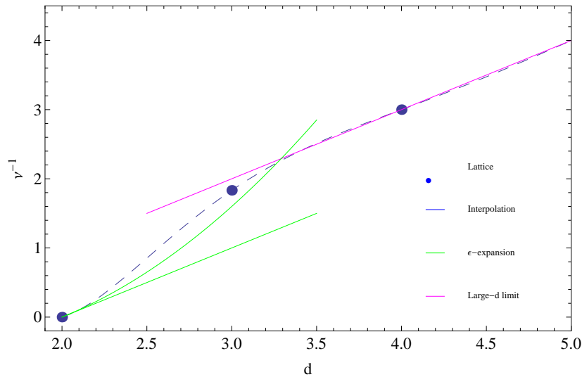
Figure 17: Universal scaling exponent \nu determining the running of G [see Eqs. (59) and (61)] as a function of spacetime dimension d . Shown are the results in 2 + 1 dimensions obtained from the exact solution of the lattice Wheeler-DeWitt equation [47], the numerical result in four dimensions (this work and [48]), the 2 + \epsilon expansion result to one [22] and two loops [23], and the large d result \nu^{-1} \simeq d - 1 [33]. For actual numerical values see Tables II and III.
