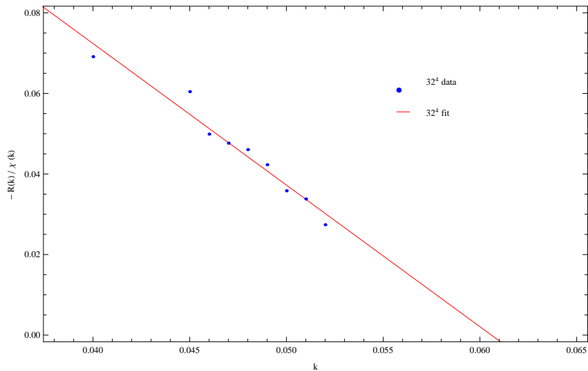
Figure 11: Inverse of the logarithmic derivative of the average curvature \mathcal{R}(k) [defined in Eq. (82)] on the 32^4 lattice with with 1,048,576 sites. The straight line represents a best fit of the form A(k_c - k) for k \geq 0.04 . The location of the critical point in k is consistent with the estimate coming from the average curvature \mathcal{R}(k) and its fluctuation \chi_{\mathcal{R}}(k) . From the slope of the line one computes directly the exponent \nu .
