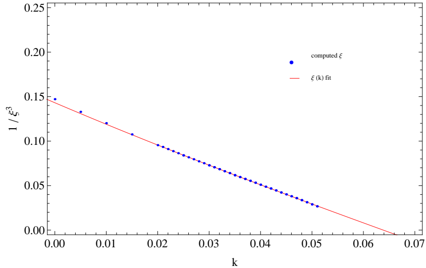
Figure 16: Estimate for the gravitational correlation length \xi(k) versus bare coupling k . For a correlation length exponent \nu = 1/3 [see Eq. (42)], 1/\xi(k)^3 is expected to be linear in k close to the critical point k_c .
