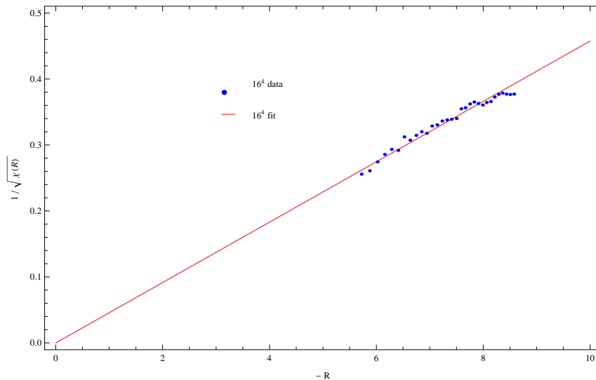
Figure 12: Inverse curvature fluctuation, 1/\sqrt{\chi_{\mathcal{R}}} , versus the average curvature \mathcal{R} . Points shown here are for the largest lattices. For \nu = 1/3 exactly, 1/\sqrt{\chi_{\mathcal{R}}} is expected to be linear in \mathcal{R} for small \mathcal{R} .
