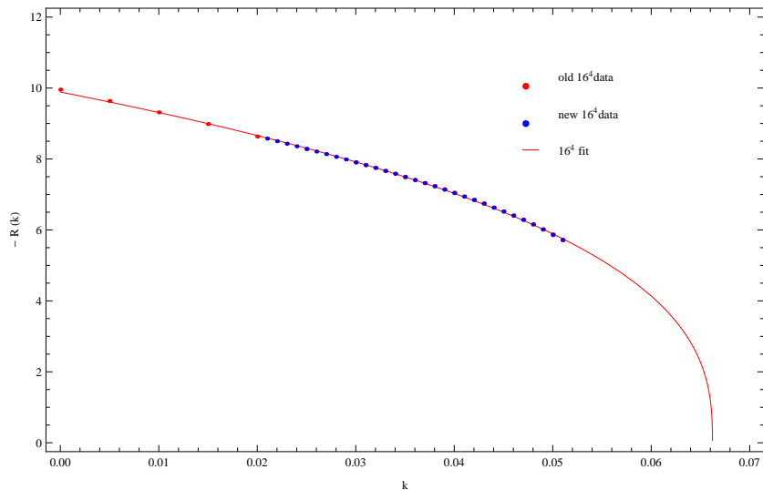
Figure 1: Average local curvature \mathcal{R}(k) as defined in Eq. (14), computed on a lattice with 16^4 = 65,536 sites. Statistical errors ( \sim \mathcal{O}(10^{-4}) ) are much smaller than the size of the symbols. The continuous line represents a fit of the form A(k_c - k)^\delta for k \geq 0.02 , with exponent \delta = 4\nu - 1 .
