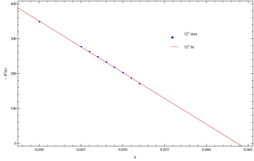
Figure 4: Average local curvature \mathcal{R}(k) on the larger 32^4 (1,048,576 sites) lattice, raised to the third power. Again if \delta = \nu = 1/3 exactly, then the points should all fall on a straight line. The continuous line represents a linear fit of the form A(k_c - k) . Deviations from linearity of the transformed data are rather small.
