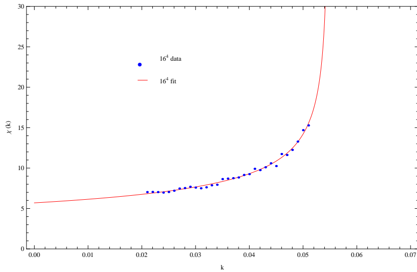
Figure 6: Curvature fluctuation \chi_{\mathcal{R}}(k) on lattices with 16^4 = 65,536 sites. The continuous line represents a fit of the form \chi_{\mathcal{R}}(k) = A(k_c - k)^{-(1-\delta)} for k \geq 0.02 .
