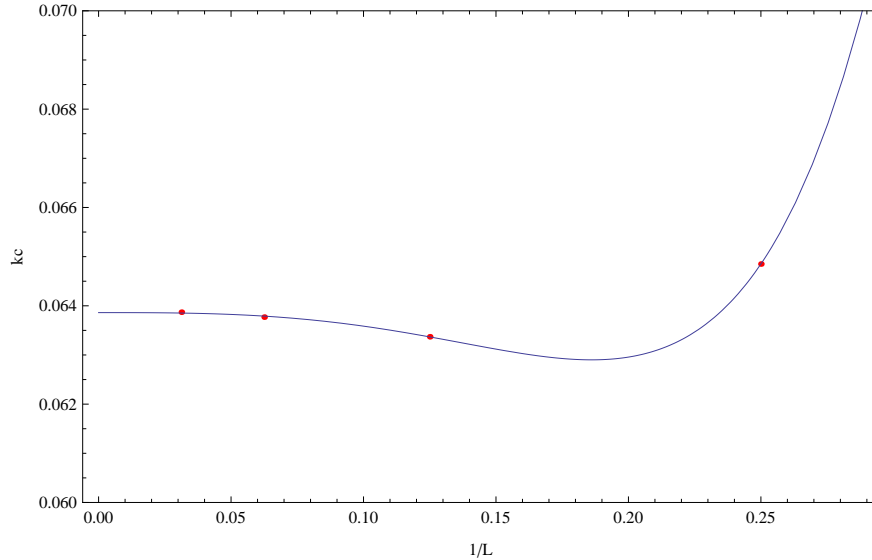
Figure 15: Size dependence of the critical point k_c(L) for different lattices, with N = L^4 sites and L = 4, 8, 16, 32 . The line represents a fit k_c(L) = k_c(\infty) + A/L^3 + B/L^6 and gives the limiting estimate k_c(\infty) = 0.0638615 .
