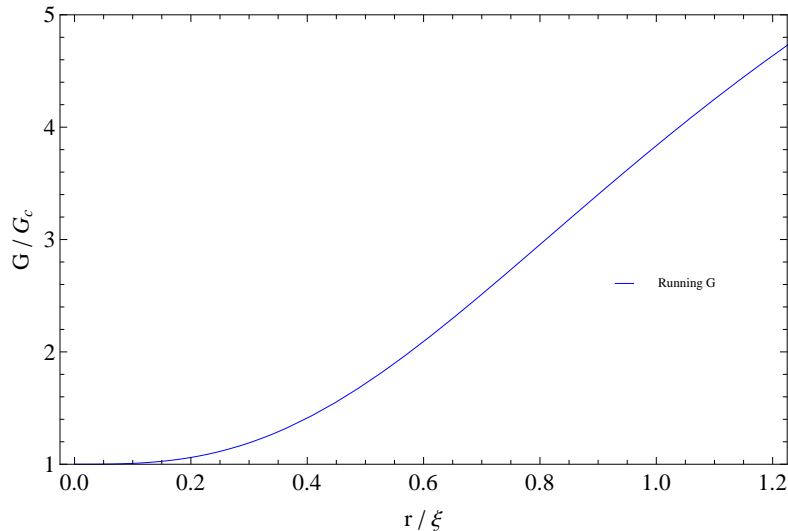
Figure 18: Running gravitational coupling G(r) versus r , obtained from the G(k) in Eq. (59) by setting k \sim 1/r , with exponent \nu = 1/3 and amplitude a_0 \simeq 8.02(55) . The lattice quantum gravity calculations done so far suggest roughly a 5% effect on scales of 0.187 \times 4890 Mpc \approx 910 Mpc , and a 10 % effect on scales of 0.238 \times 4890 Mpc \approx 1160 Mpc .
