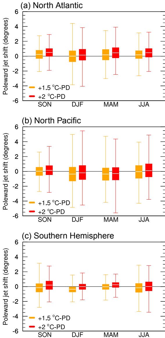
Figure 6. Multi-model mean shift of the eddy-driven jet in the 1.5 °C (orange) and 2.0 °C (red) experiments relative to the PD experiment for each season (a) North Atlantic sector (60° W–0), (b) North Pacific sector (135–235° E), and (c) Southern Hemisphere. The white horizontal line in the boxes indicates the median, the boxes indicate the interquartile range, and the whiskers indicate the spread across all ensemble members for all models. Jet latitude is determined according to the method of Woollings et al. (2010). The mean shifts are very close to, but different from, zero based on 95 % confidence intervals from 10 000 bootstrapped realisations of the full HAPPI ensemble (926 members over all models), with the exception of the following seasons/sectors: for 1.5 °C–PD, North Atlantic DJF, North Pacific JJA/SO, Southern Hemisphere MAM; for 2.0 °C–PD, North Pacific DJF/JJA/SO, Southern Hemisphere DJF/JJA.
