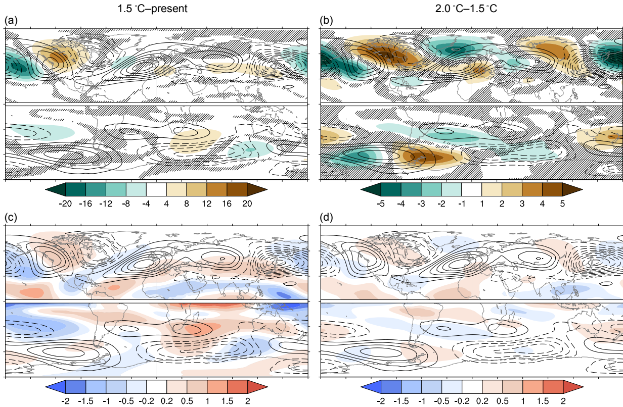
Figure 10. Multi-model mean response of winter (Northern Hemisphere DJF, Southern Hemisphere JJA) stationary waves at 500 hPa for 1.5°C–PD ( a , c ) and 2.0–1.5°C ( b , d ). Panels ( a ) and ( b ) show responses (shading; units m) along with the climatology (contour interval 25 m) for the ( a ) PD and ( b ) 1.5°C experiments. Note the different colour scale for ( a ) and ( b ). Panels ( c ) and ( d ) show signal-to-noise ratio \beta/\sigma , where the sign corresponds to the sign of the response, along with the climatology (contour interval 25 m) for the ( c ) 1.5°C and ( d ) 2.0°C experiments. In ( a ) and ( b ), hatching masks out regions where there is no model consensus (fewer than four out of five models agree) on the sign of the response. In ( c ) and ( d ), black dots mask out regions where the models do not agree on the magnitude of the response ( f^2 > 1 ). Stationary waves are defined as departures from the zonal mean of geopotential height ( Z^* ) at 500 hPa.
