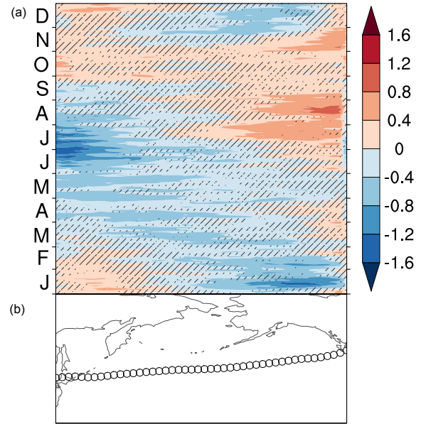
Figure 7. (a) Multi-model mean shift of the North Pacific eddy-driven jet (shading; in degrees latitude) in the 2.0 °C experiment compared to the PD experiment as a function of longitude and time. Hatching masks out regions where there is no model consensus (fewer than four out of five models agree) on the sign of the response. (b) Climatological position of the jet in the PD experiment. Jet latitude is calculated following Simpson et al. (2014).
