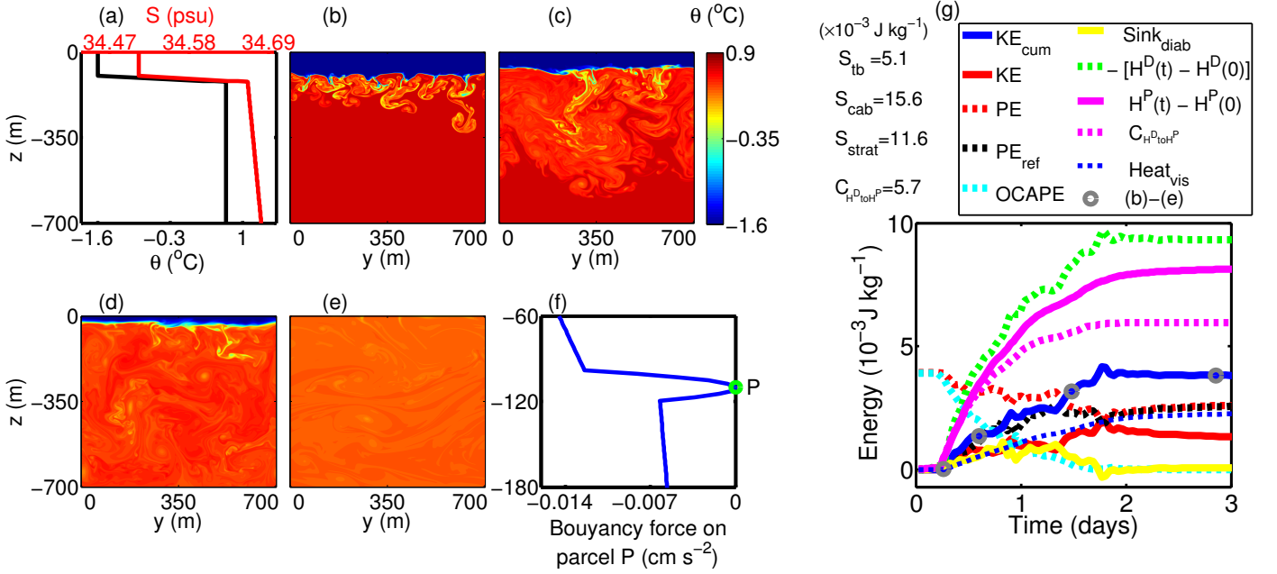
FIG. 5. As Figure 2, except panel (f), for a stratified simulation with cabbeling included in the EOS. This is case 4.4 of Table 4 discussed in section 4d. It adopts the full nonlinear EOS of seawater (Jackett et al. 2006) and a detailed model configuration is described in Table 4. Snapshots of the model’s \theta ( ^{\circ}\text{C} ) are shown (b) at t=0.26 day, (c) at t=0.59 day, (d) at t=1.49 days, and (e) at t=2.8 days. Panel (f) follows Figure 9(b) of Harcourt (2005): it shows the buoyancy force on parcel P using the full nonlinear EOS when it is displaced vertically and adiabatically across the initial profile. Parcel P is originally located at the depth of 115 m within the initial interface (100-120 m depths). Panel (f) suggests a cabbeling instability when moving parcel P downward, since it becomes negatively buoyant. For (g), see Figure 1 for the detailed energy relations.
