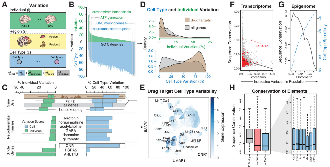
Figure 3. Measuring transcriptome and epigenome variation across the cohort at the single-cell level.
