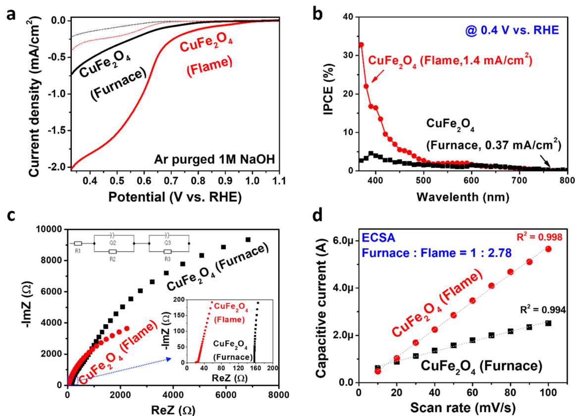
Figure 4. Photoelectrochemical (PEC) characterizations on CuFe 2 O 4 photocathode by furnace and flame. (a) J - V curves of CuFe 2 O 4 photocathode measured in Ar purged 1 M NaOH under simulated 1 sun illumination (100 mW/cm 2 ) for hydrogen production. The scan rate was 10 mV/s and the scan direction was in cathodic sweep. (b) Incident photon to current efficiency (IPCE) of CuFe 2 O 4 photocathode. (c) Electrochemical impedance spectra (EIS) of CuFe 2 O 4 photocathode at 0.4 V vs RHE under simulated 1 sun illumination. (d) Capacitive currents measured at 1.13 V vs RHE as a function of scan rate for the relative electrochemical active surface area (ECSA) measurements. In all figures, CuFe 2 O 4 (Furnace) is black and CuFe 2 O 4 (Flame) is red.
