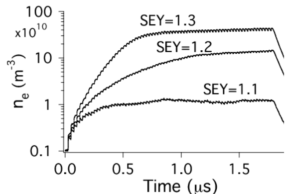
Figure 1: Average electron density versus time at a given station in the SPS (from a POSINST simulation).
