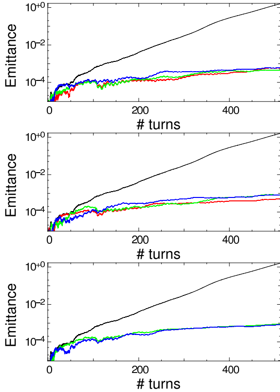
Figure 3: Beam emittance versus turn number from Warp simulations of a 120 GeV beam in the SPS with an initial background of electrons of 1 \times 10^{12} m^{-3} , with no feedback (black), feedback 1 (red), feedback 2 (green), and feedback 3 (blue), and with (top) no weighting, no filter, (middle) weighting, no filter, (bottom) weighting, lowpass filter with cutoff at 1GHz
