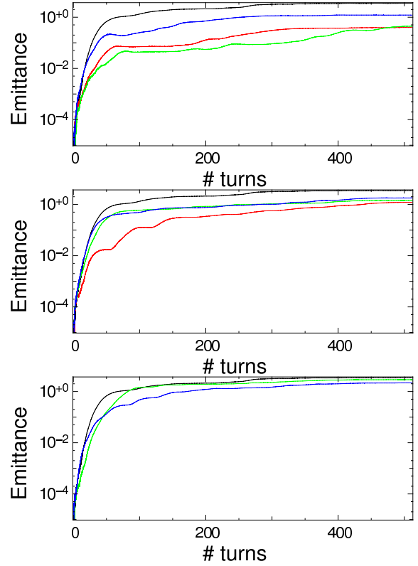
Figure 4: Same as Fig.3, but with an initial background of electrons of 5 \times 10^{12} m^{-3} .
