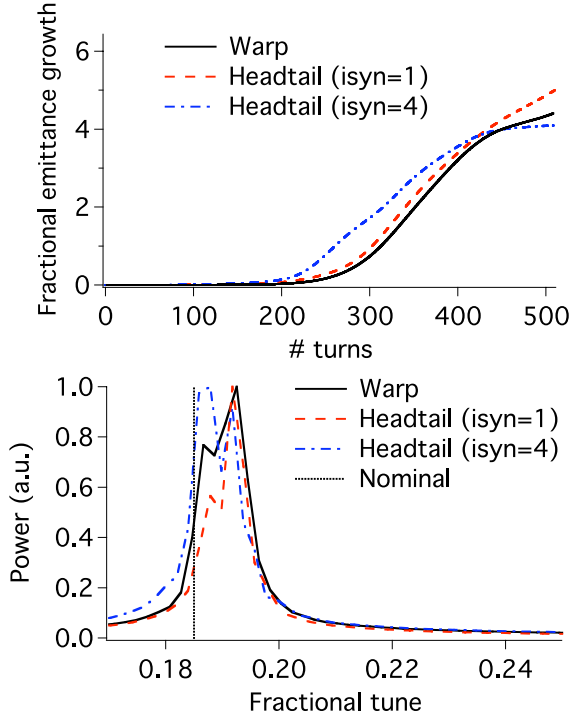
Figure 2: Beam emittance versus turn number (top) and normalized power versus fractional tune (bottom) from computer simulations of electron cloud driven instability using the codes Warp and Headtail. On the bottom plot, a dotted line indicates the location of the nominal vertical fractional betatron tune (0.185).
