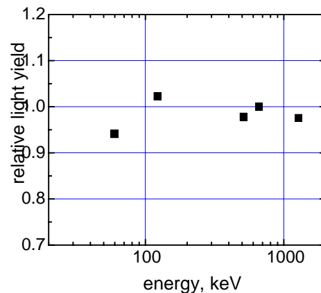
Fig. 5. Energy response (relative light yield, normalized to the value at 662 keV, as a function of energy) for LaCl 3 :10%Ce. The response of an ideal material would be independent of energy. Non-proportionality of measured sample is ~7% which is much better than that in established scintillators.
