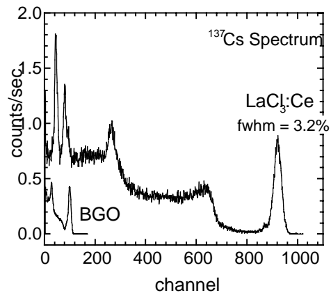
Fig. 1. ^{137}\text{Cs} spectra recorded with \text{LaCl}_3:10\%\text{Ce} and BGO crystals coupled to PMT under identical operating conditions. Light output of \text{LaCl}_3:10\%\text{Ce} was estimated to be \sim 50,000 photons/MeV from the calibration provided by BGO. The \text{LaCl}_3 spectrum shows resolution of 3.2% (FWHM) at room temperature.
